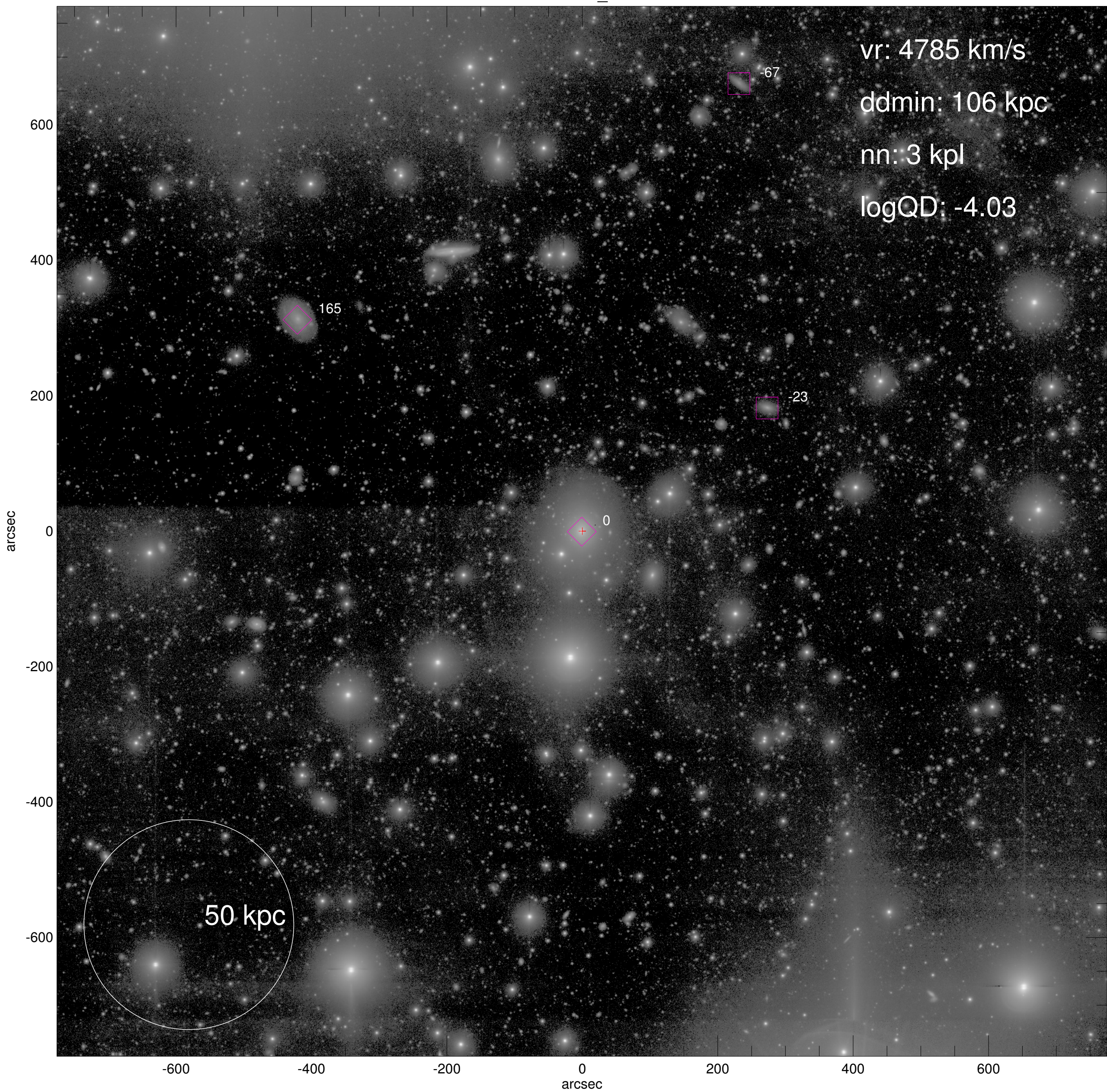
NGC7198_wide
