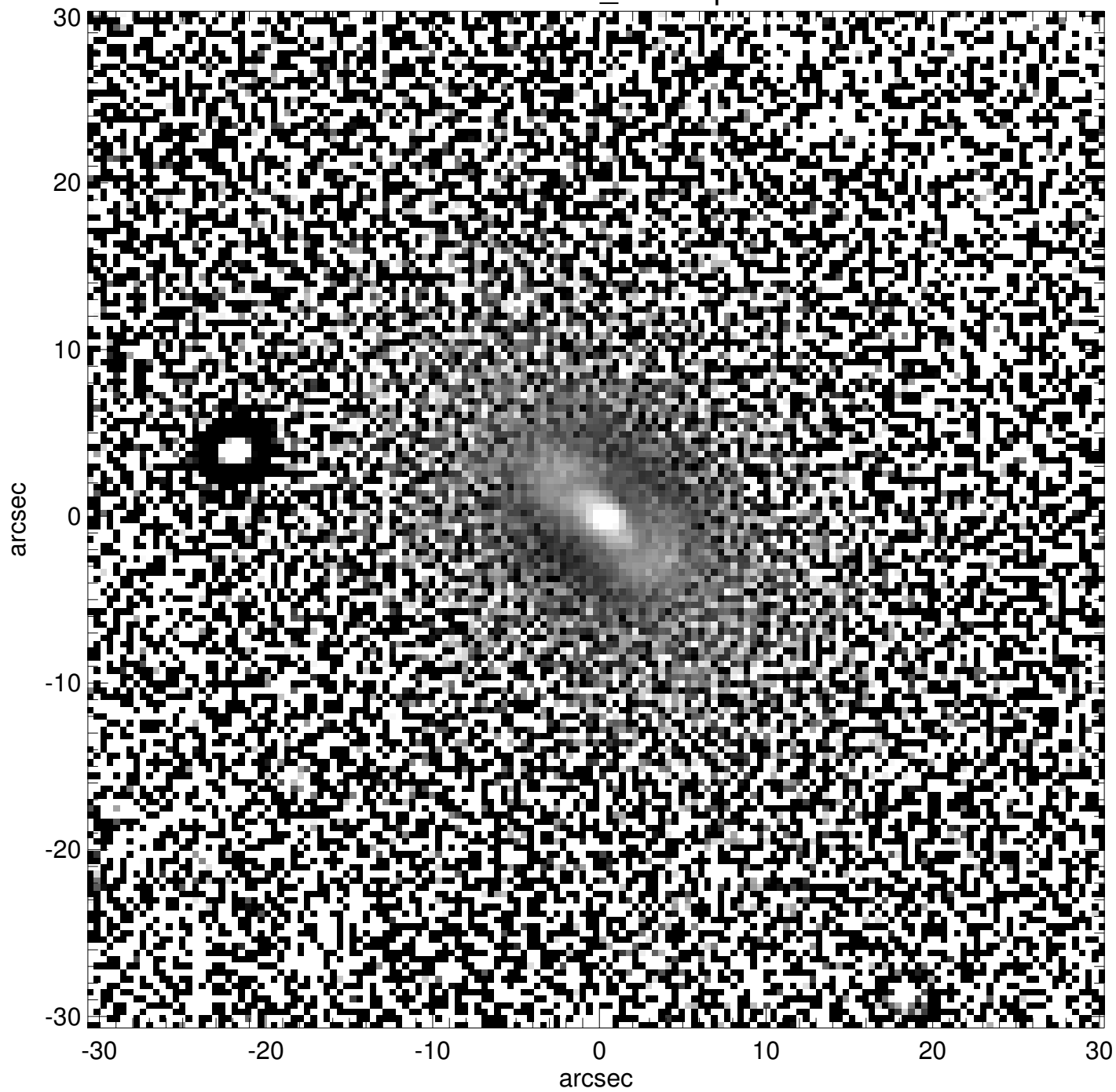
NGC7402_unsharp
