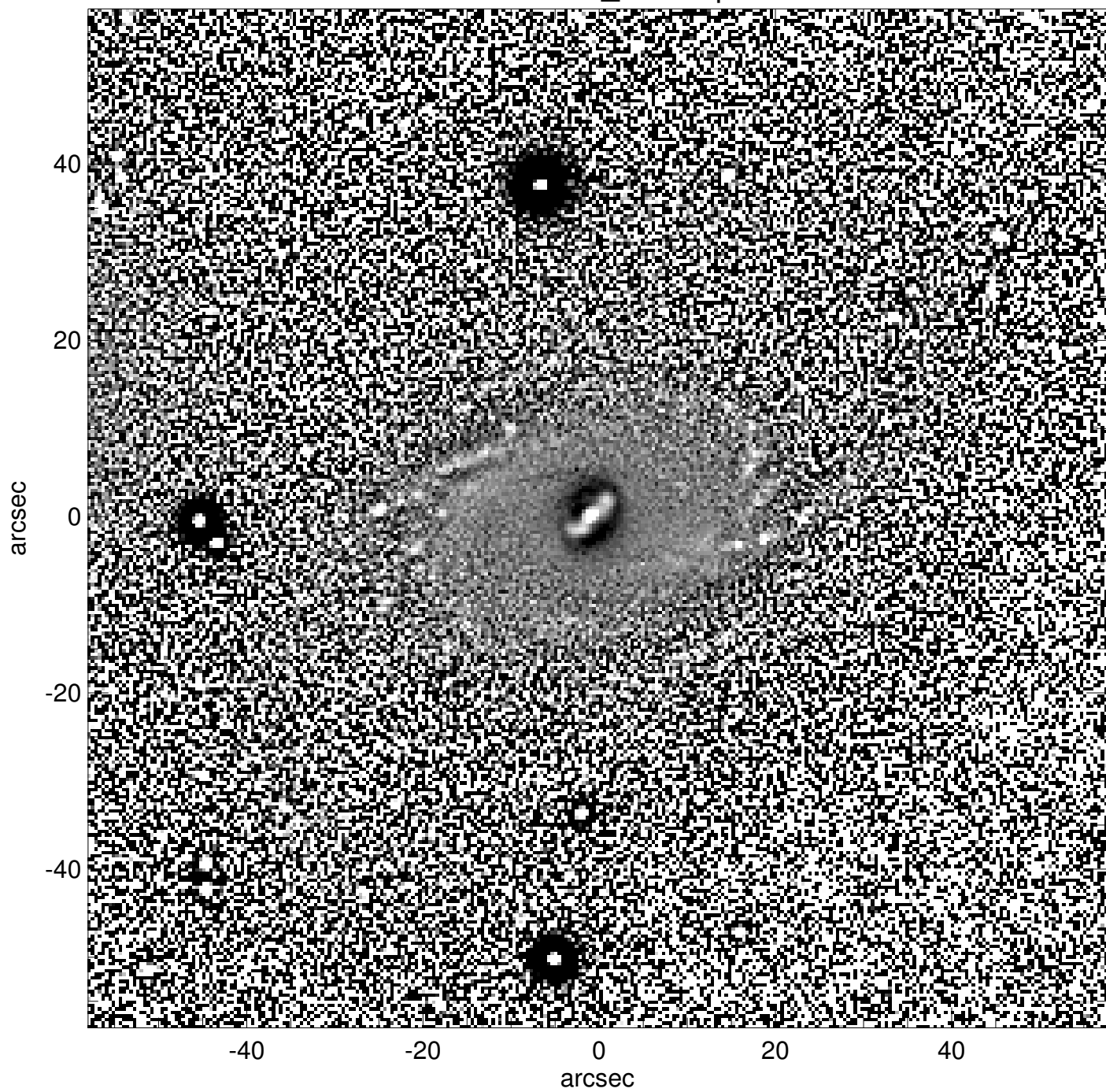
NGC7589_unsharp
