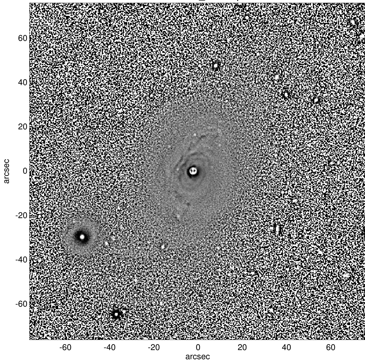
NGC7603_unsharp
