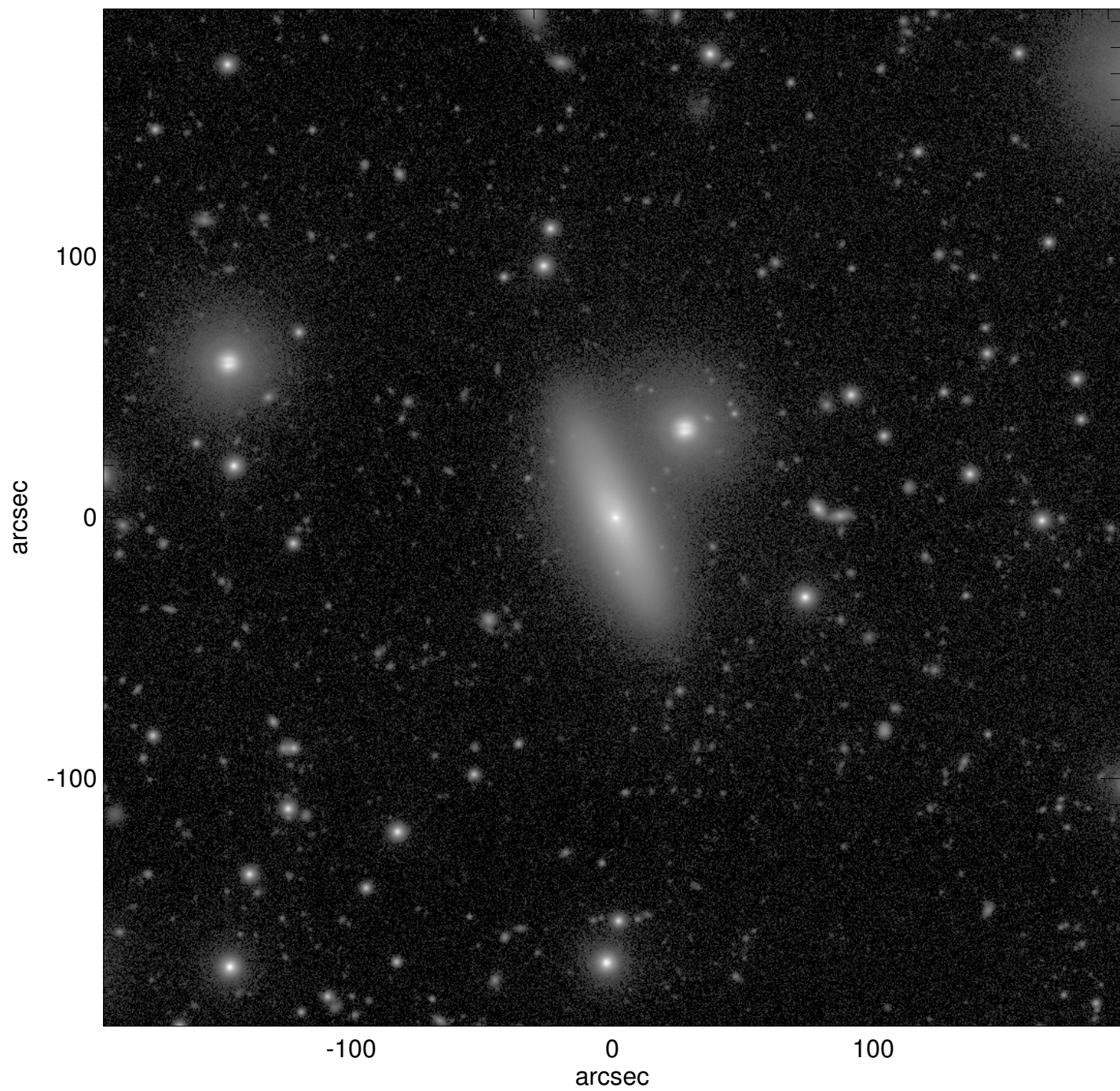
NGC7684
