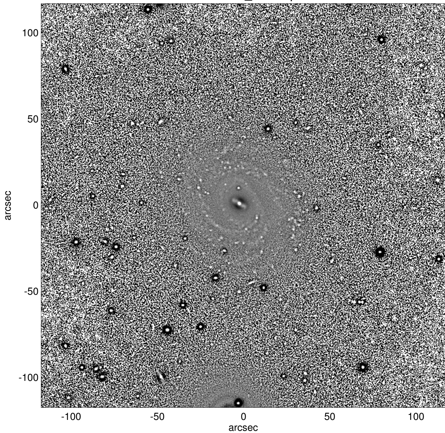
NGC7716_unsharp
