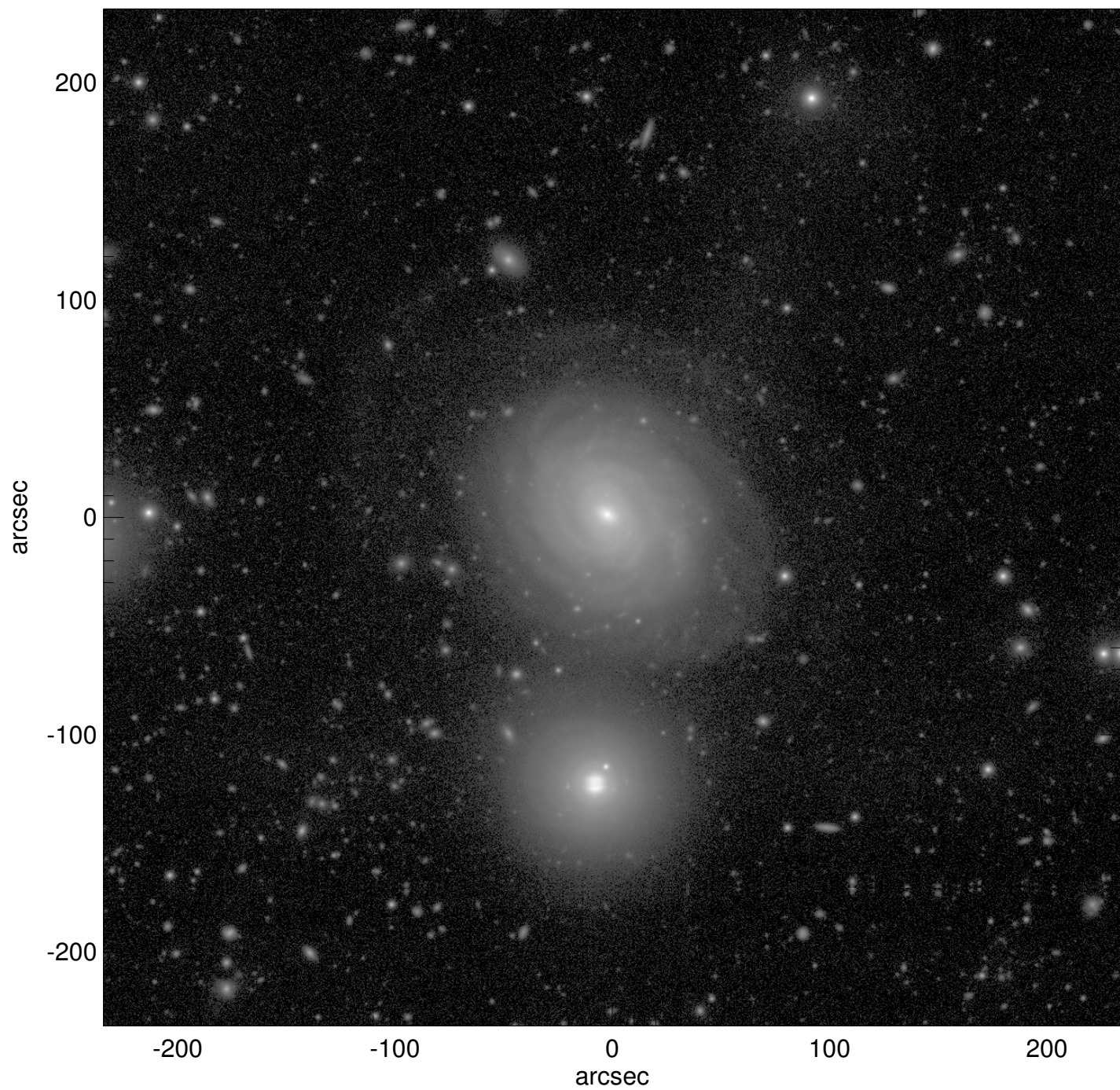
NGC7716
