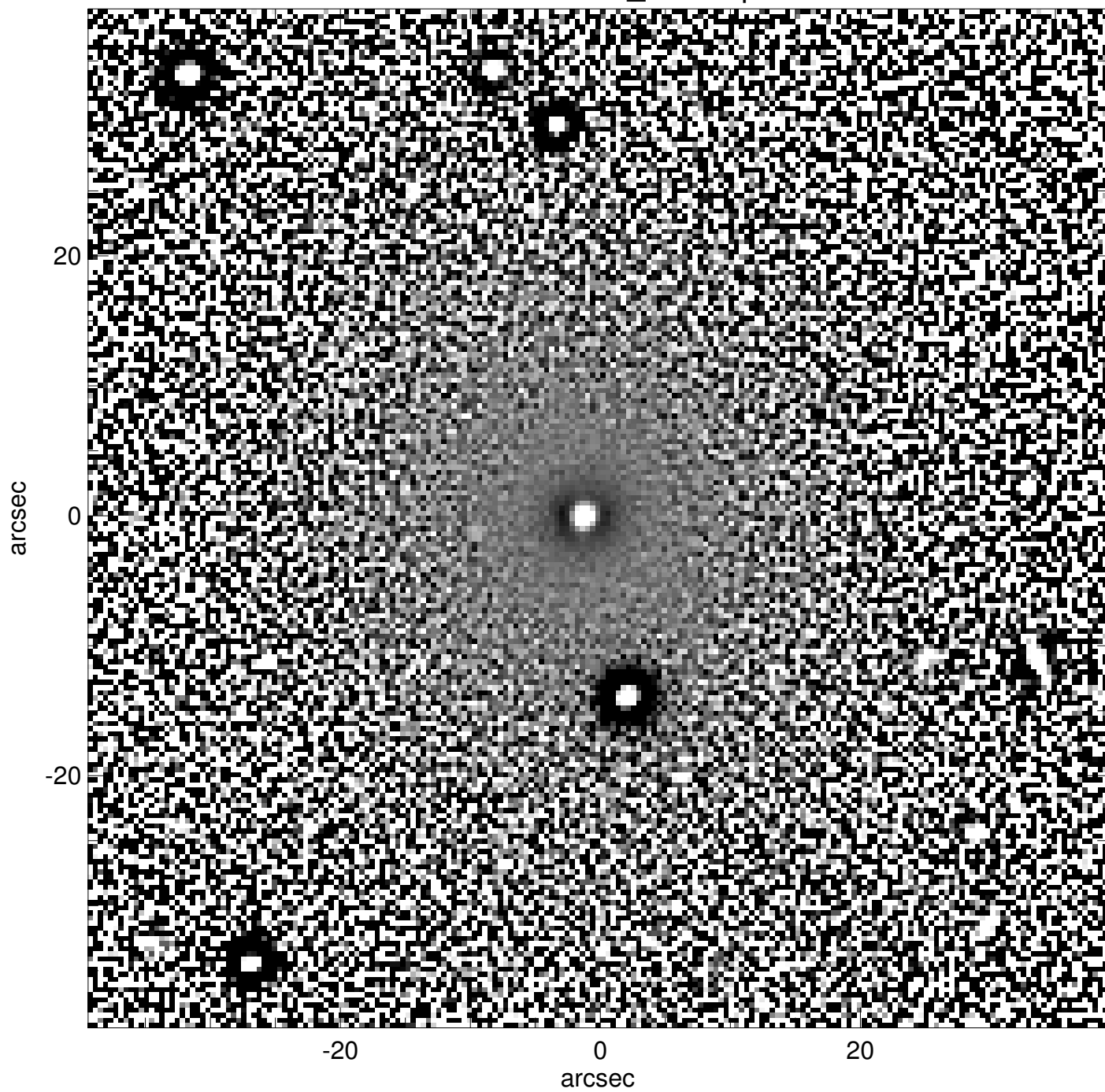
PGC0001505_unsharp
