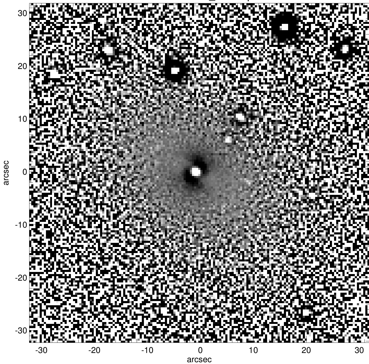
PGC0072050_unsharp
