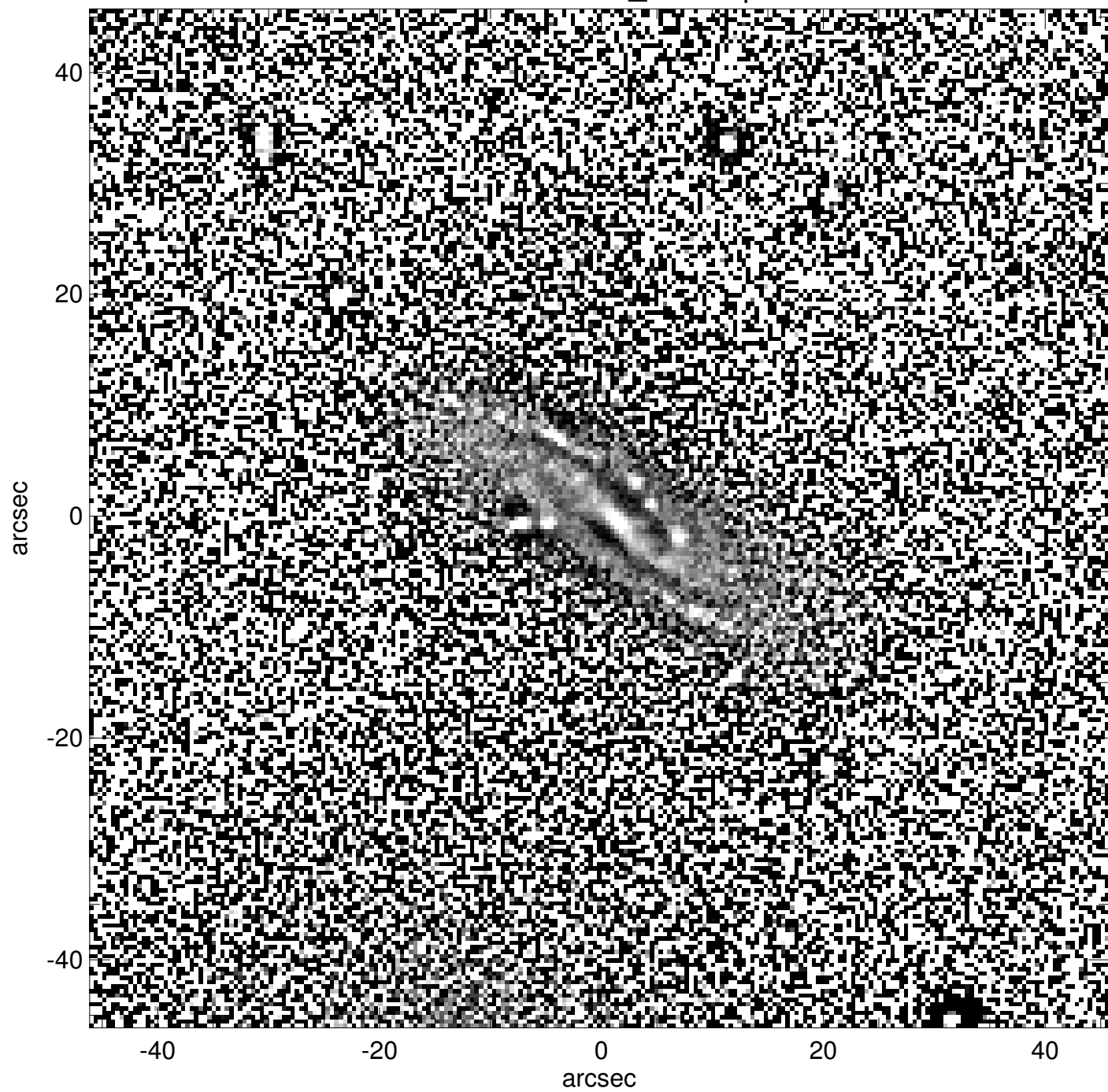
PGC0072913_unsharp
