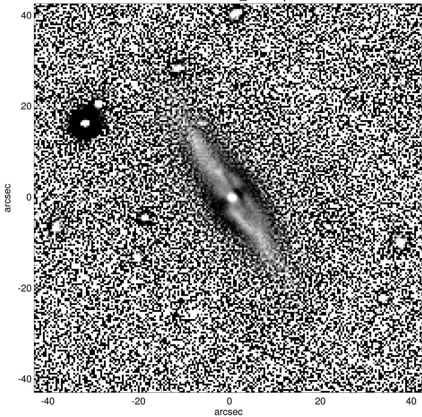
PGC0212799_unsharp
