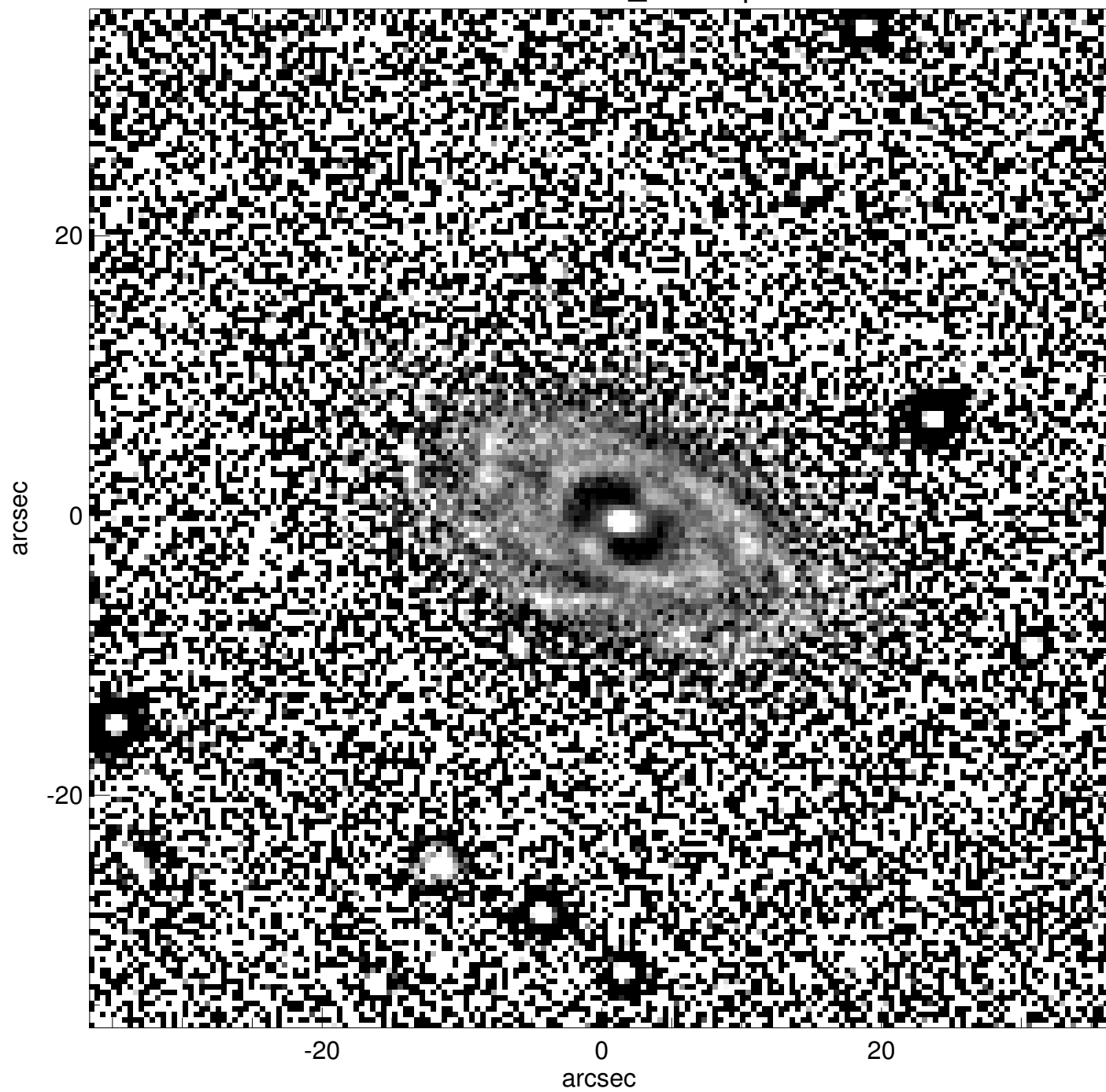
PGC1125254_unsharp
