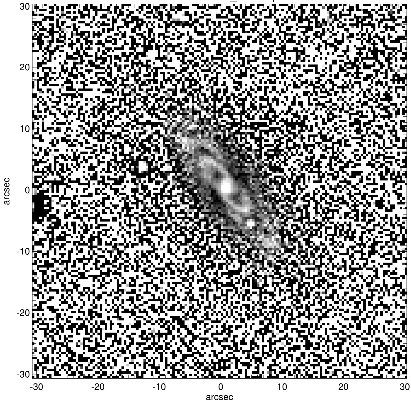
PGC1134911_unsharp
