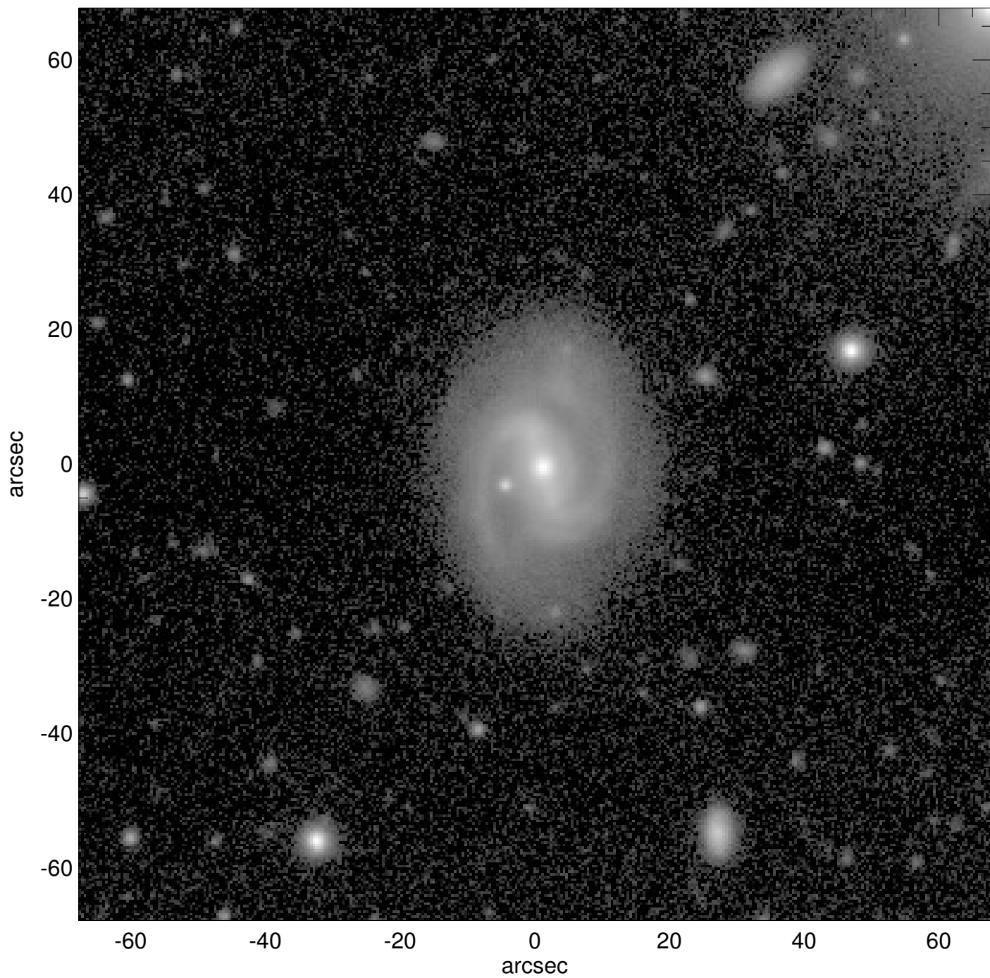
PGC1137099
