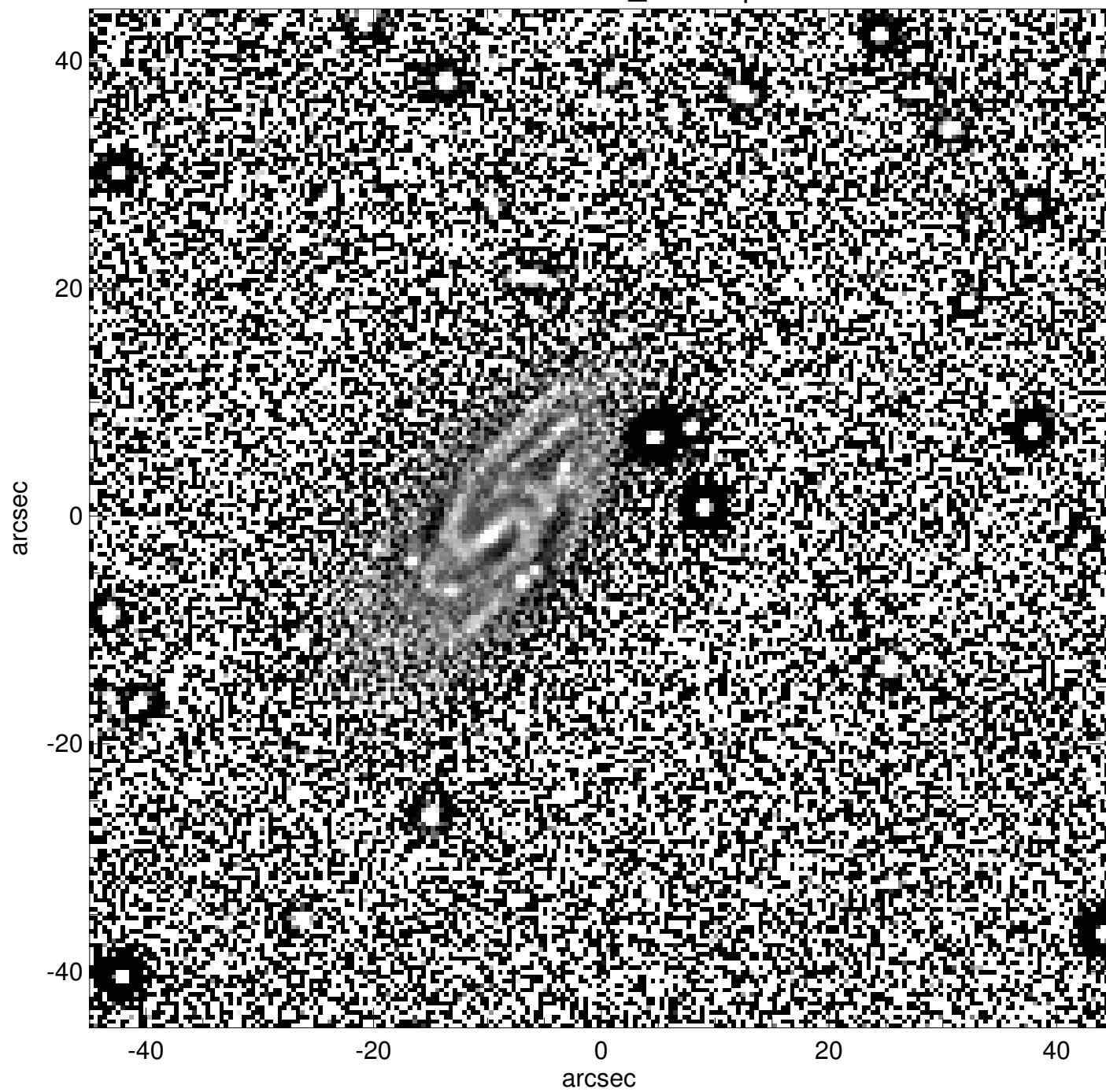
PGC1142473_unsharp
