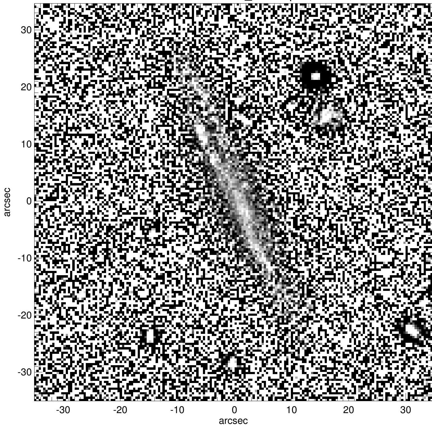
PGC1143006_unsharp
