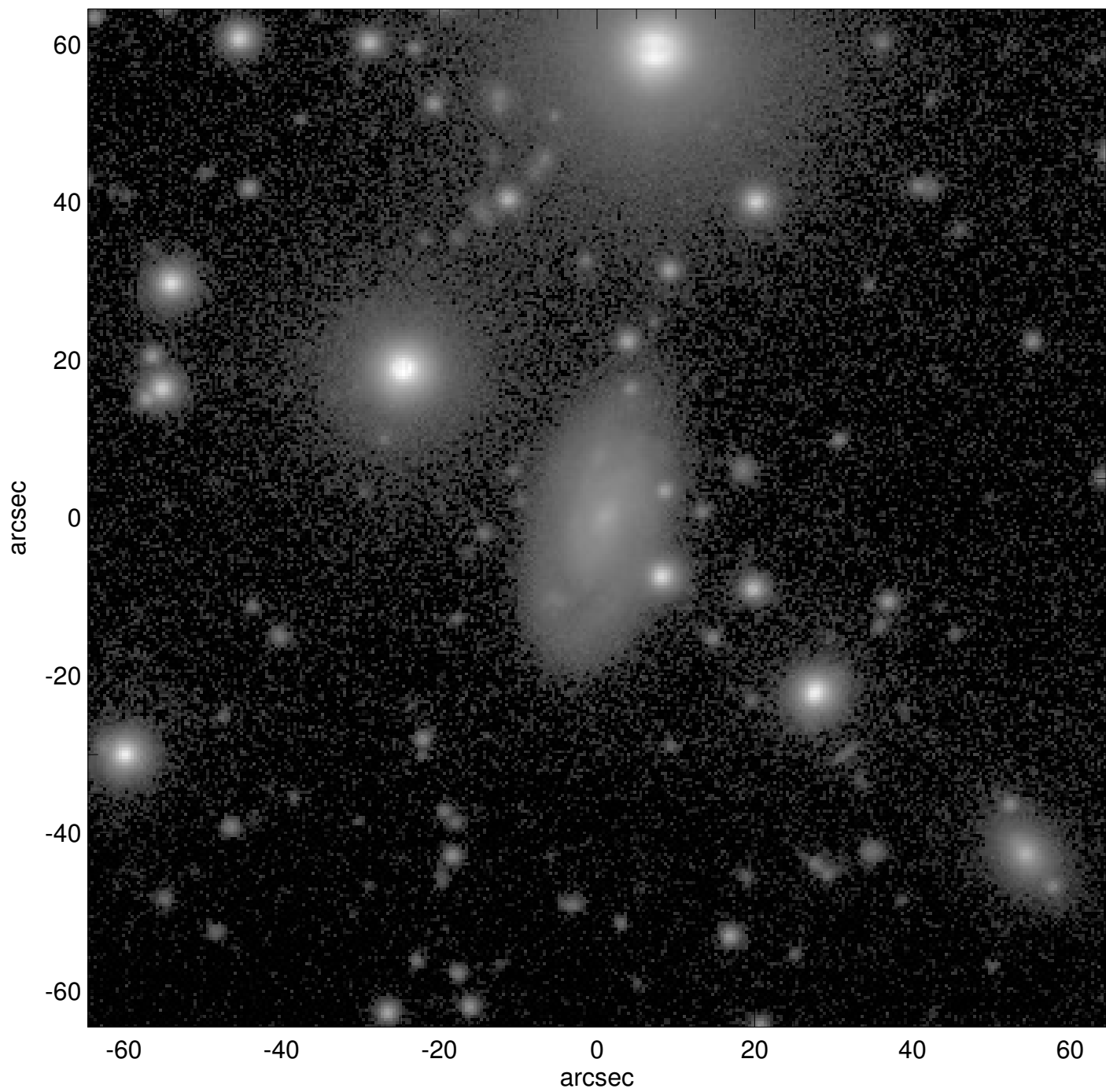
PGC1144230
