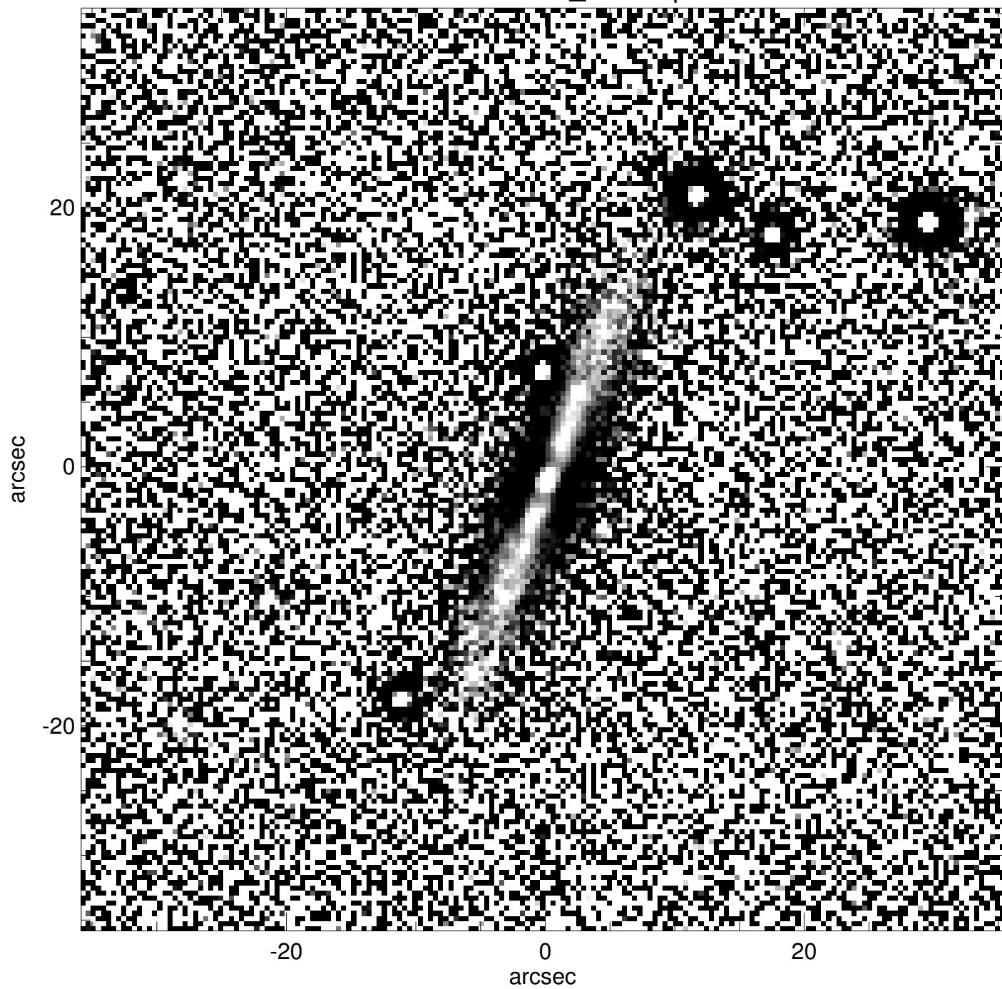
PGC1144700_unsharp
