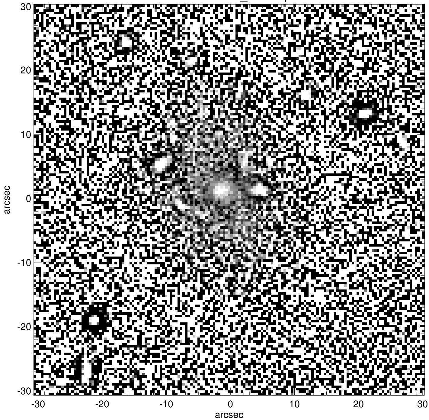
PGC1147712_unsharp
