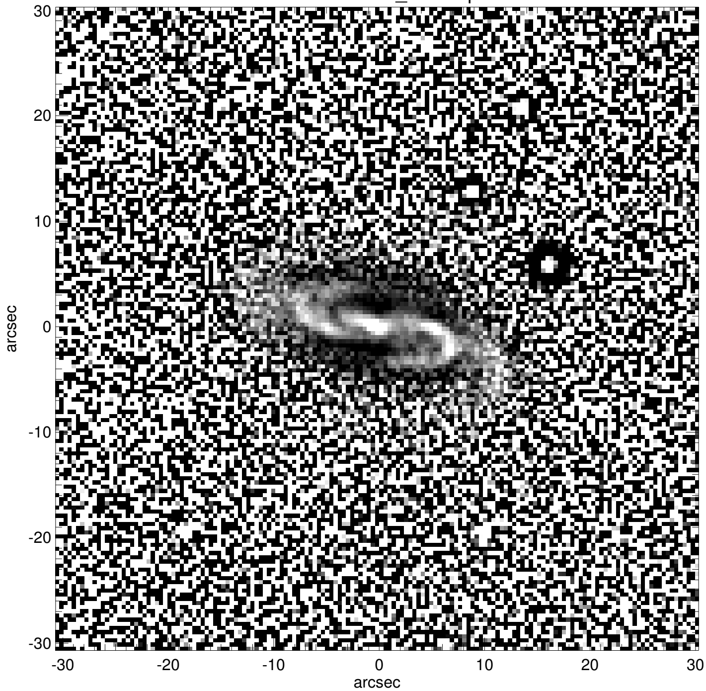
PGC1149898_unsharp
