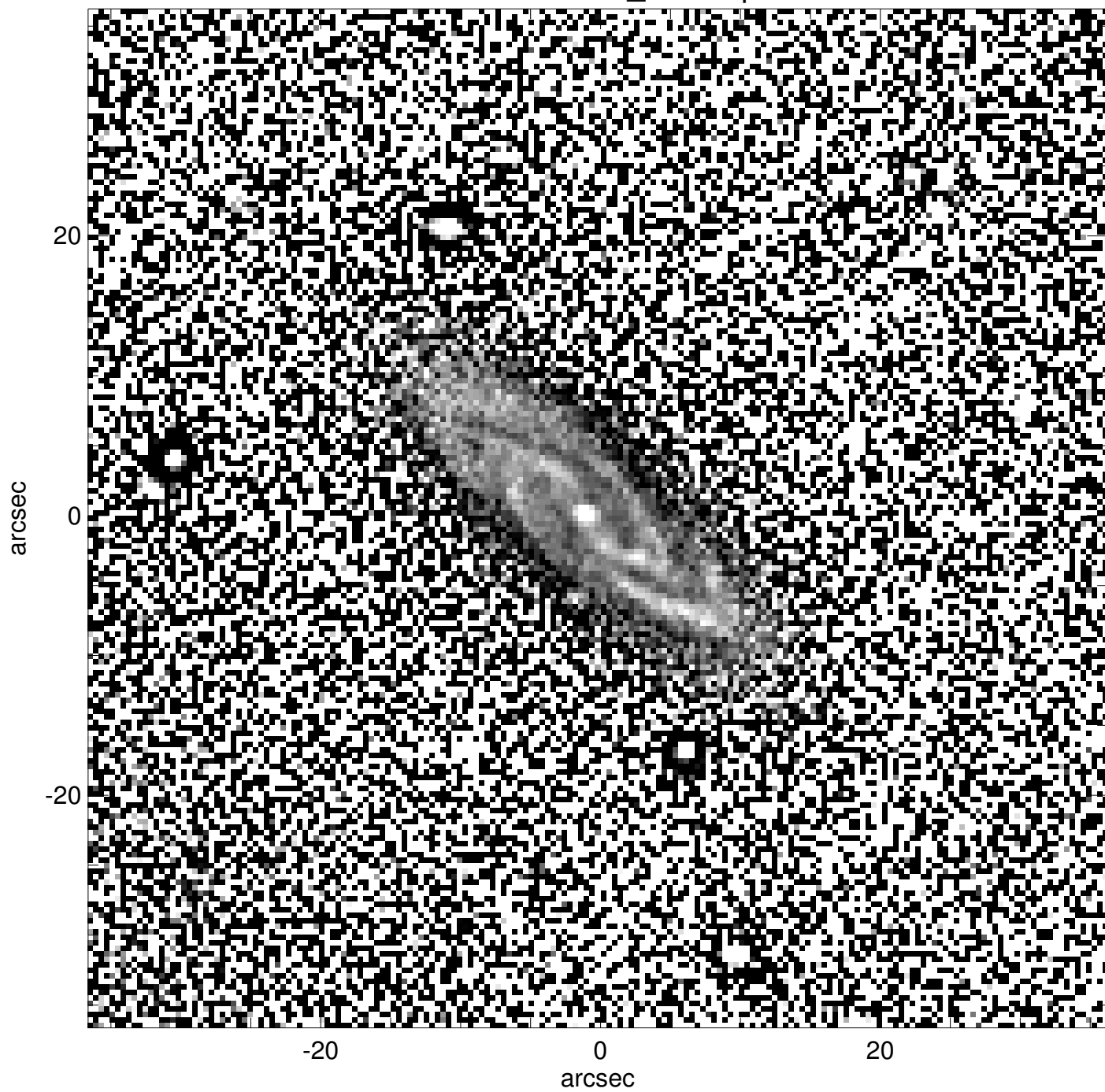
PGC1159036_unsharp
