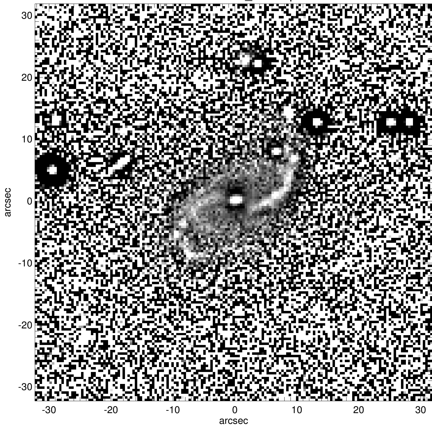
PGC1163881_unsharp
