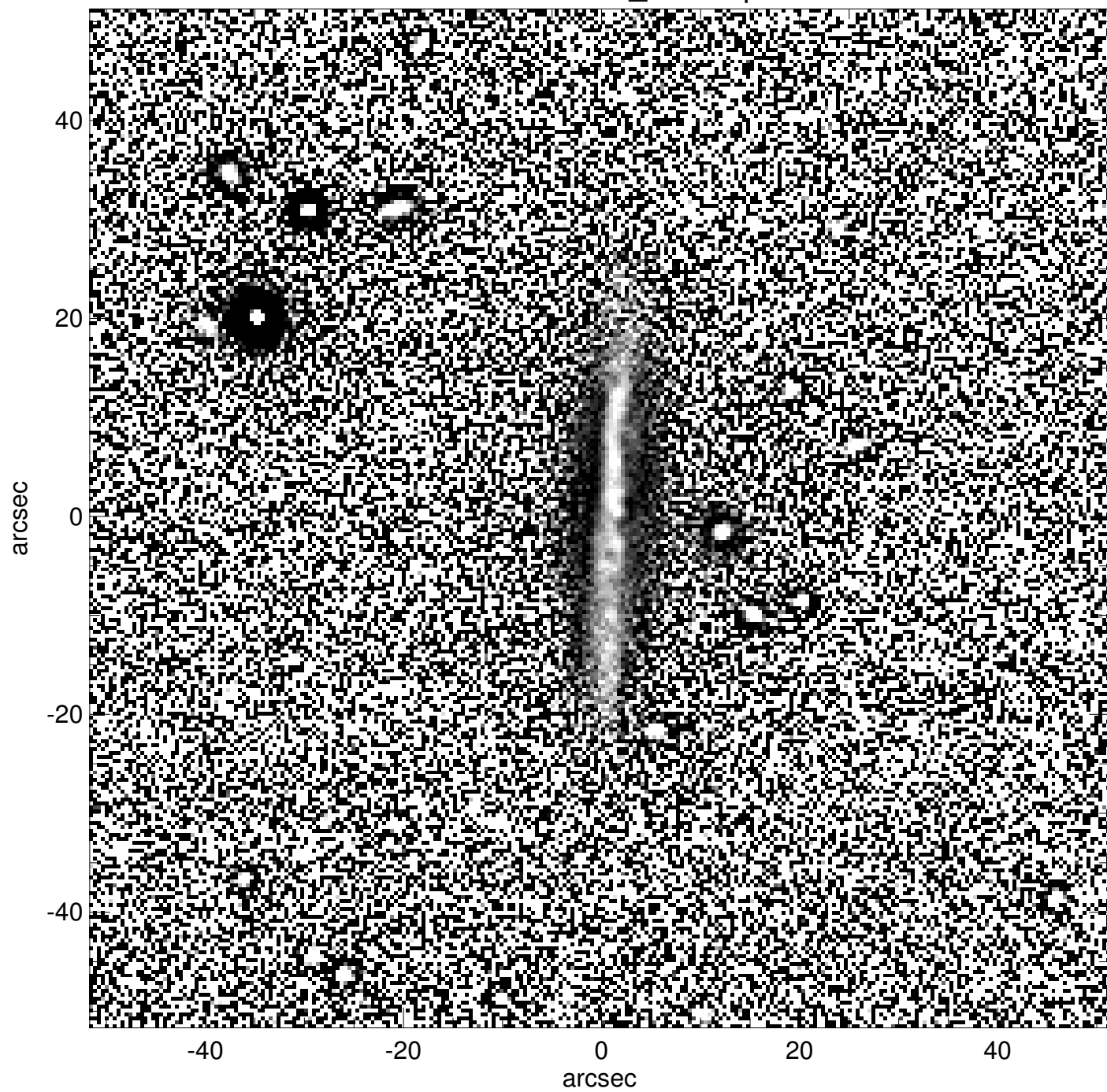
PGC1166532_unsharp
