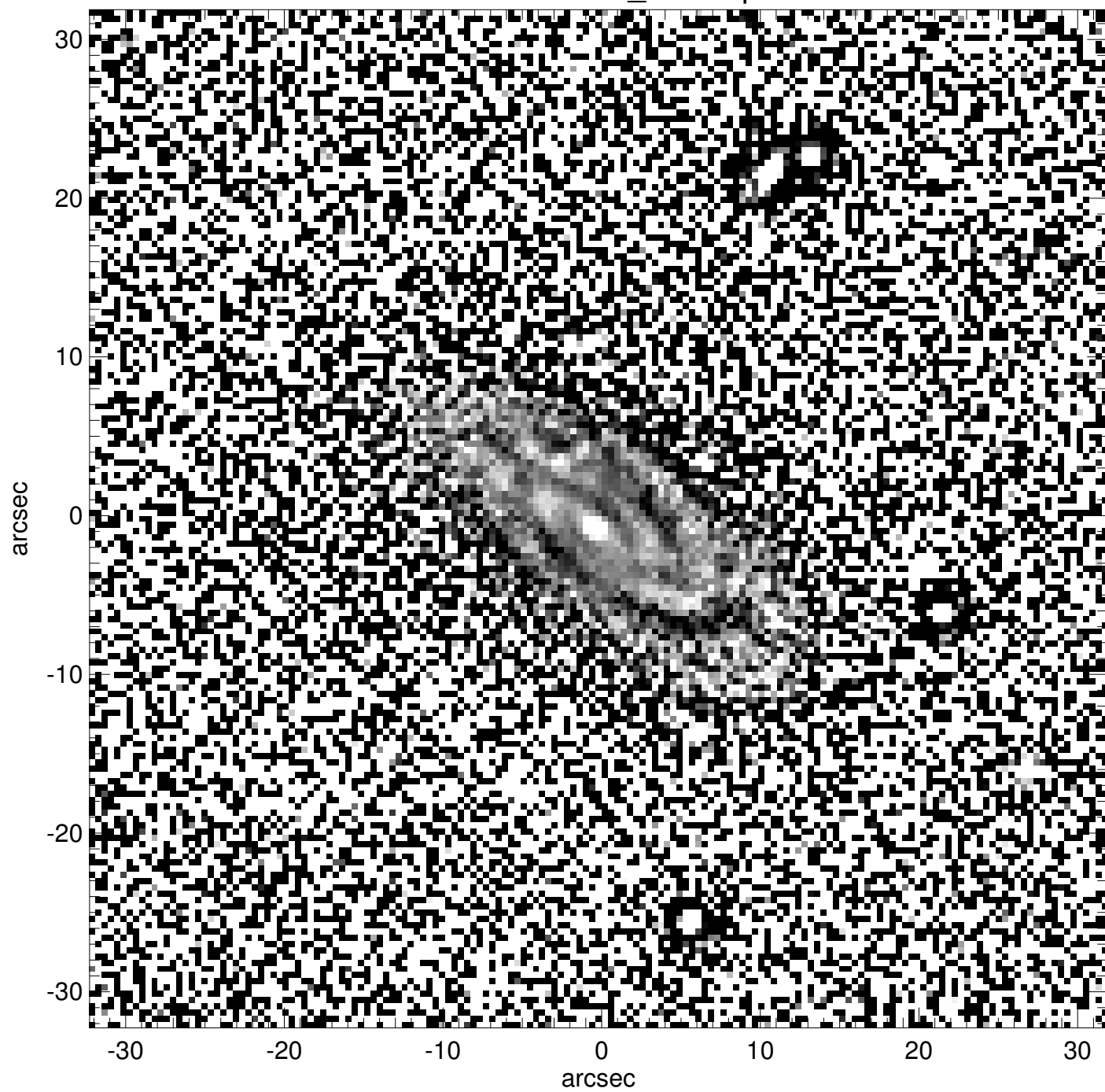
PGC1169116_unsharp
