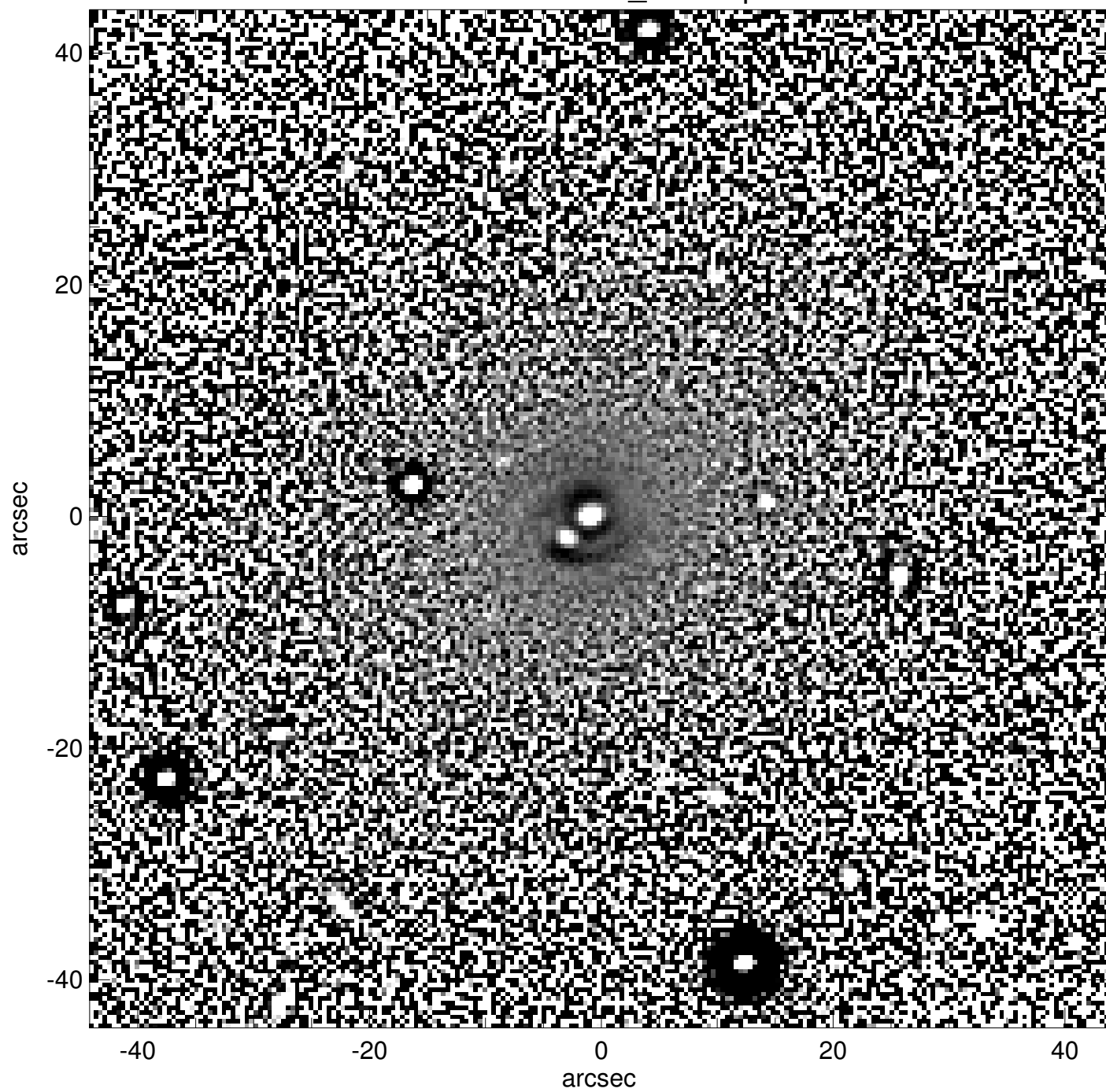
PGC1175702_unsharp
