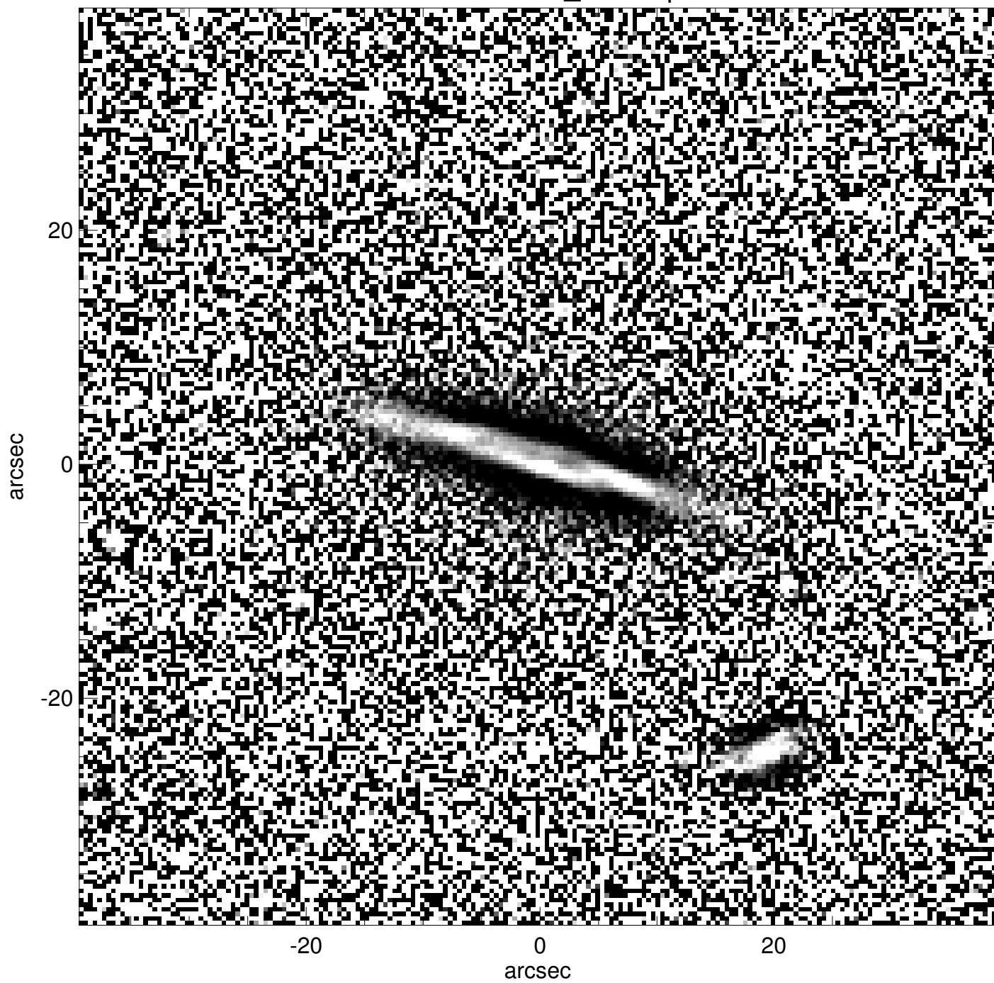
PGC1180460_unsharp
