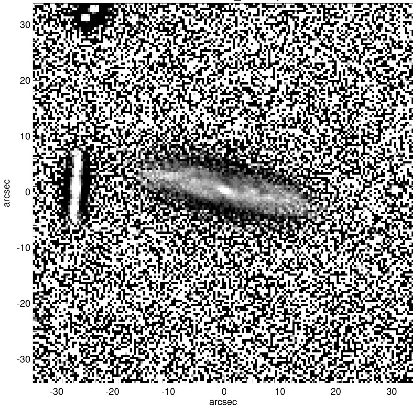
PGC1183073_unsharp
