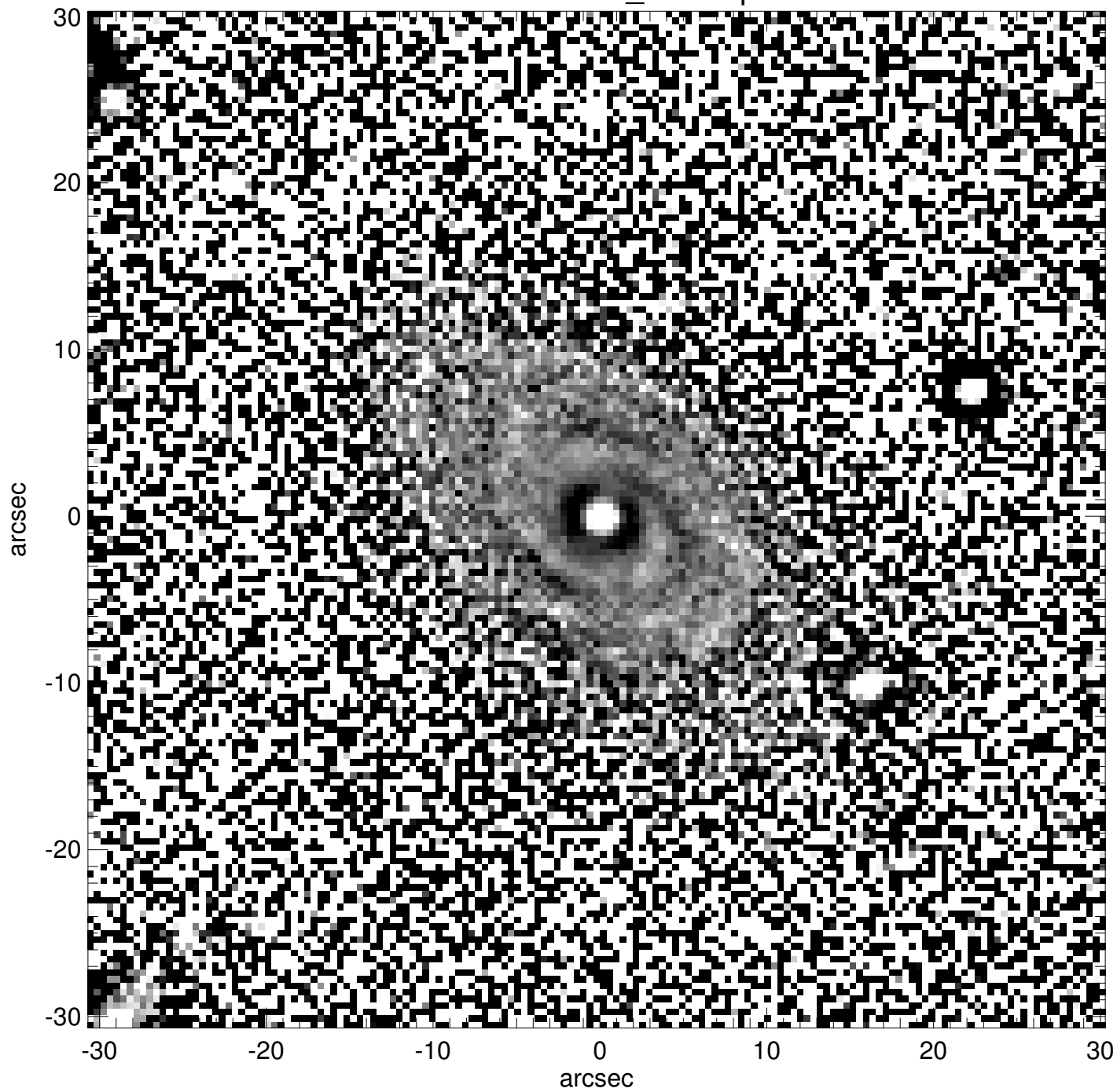
PGC1183248_unsharp
