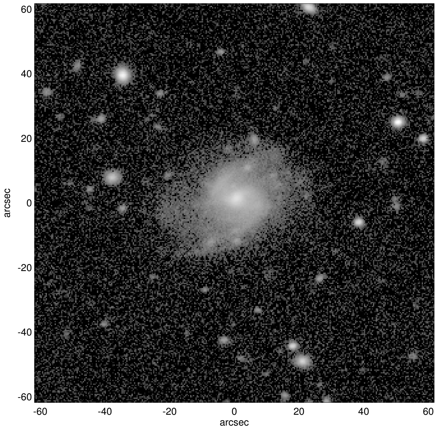
PGC1185880
