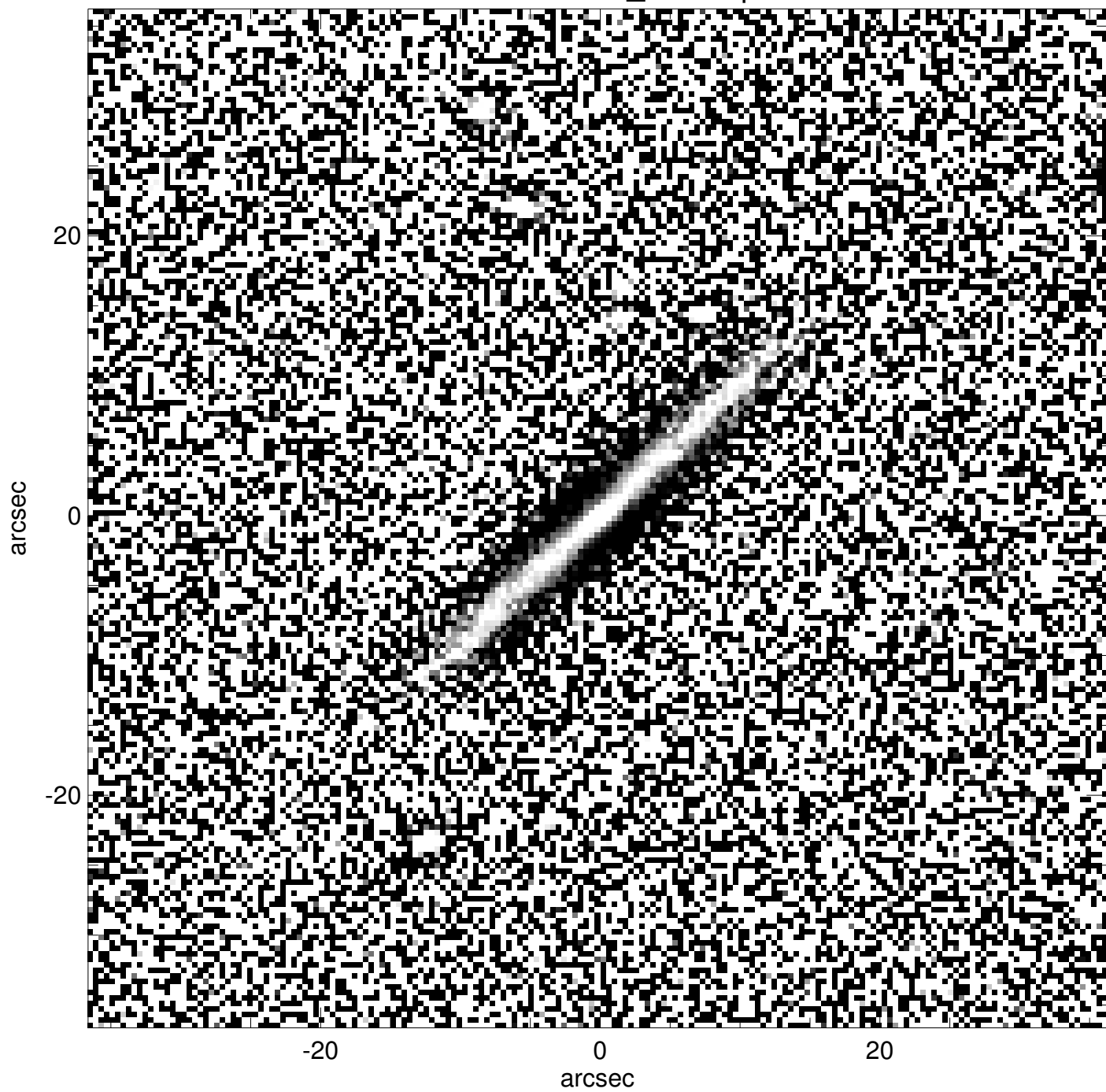
PGC1185888_unsharp
