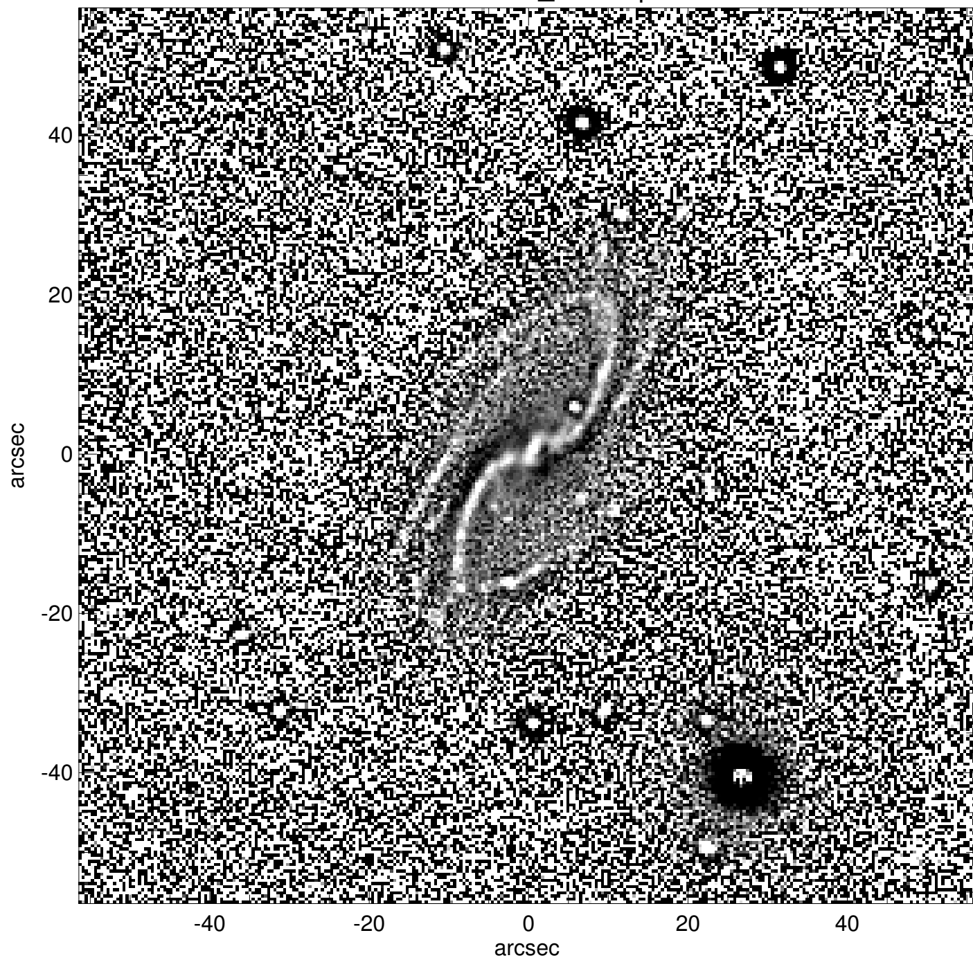
UGC00295_unsharp
