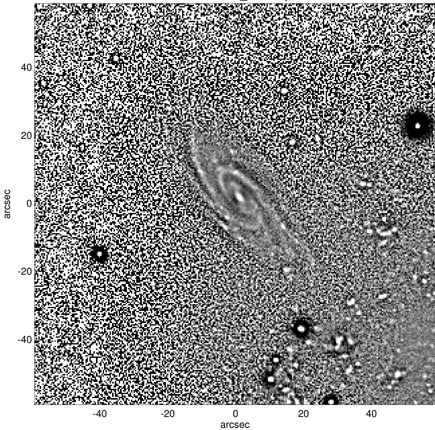
UGC00807_unsharp
