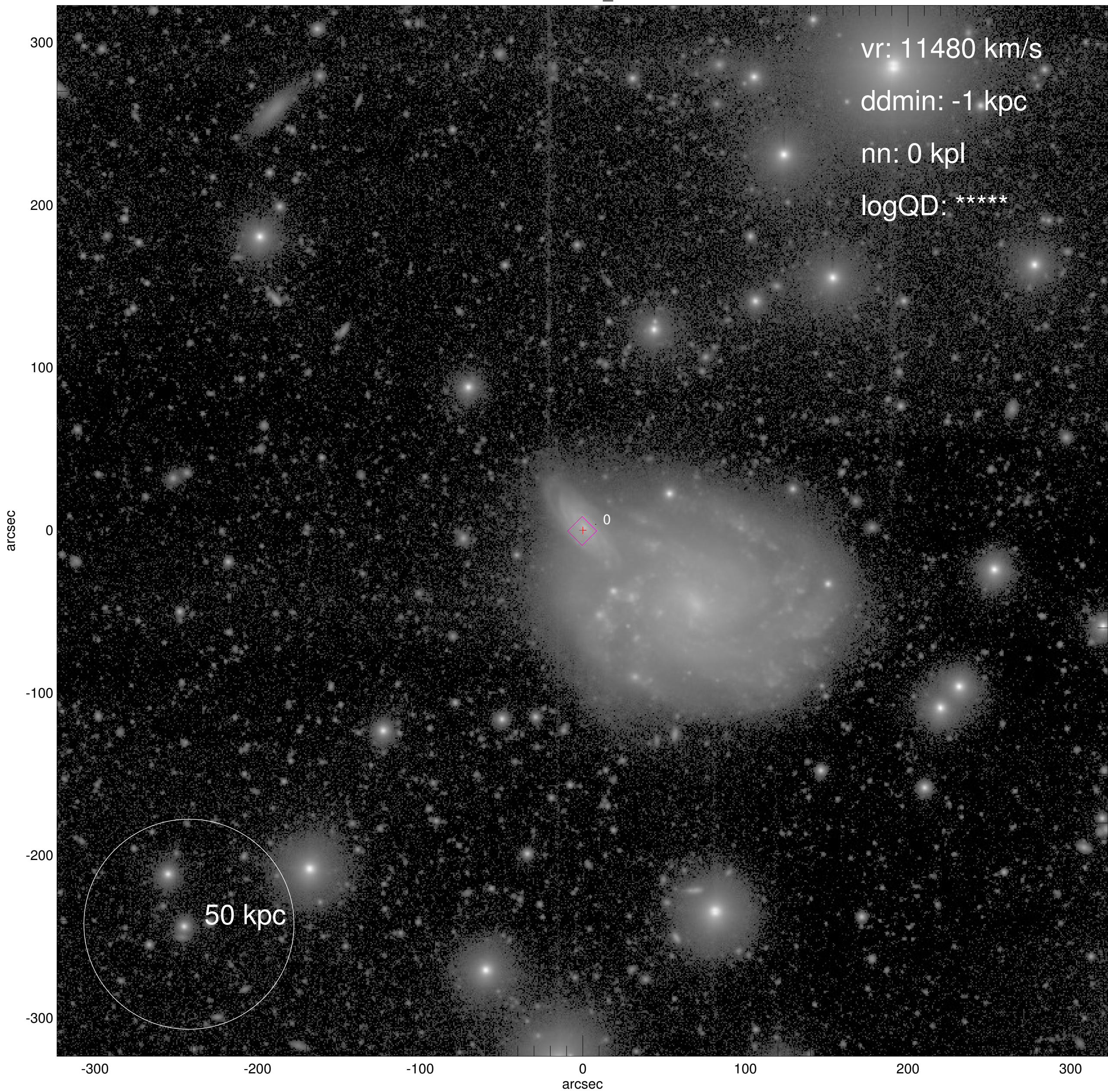
UGC00807_wide
