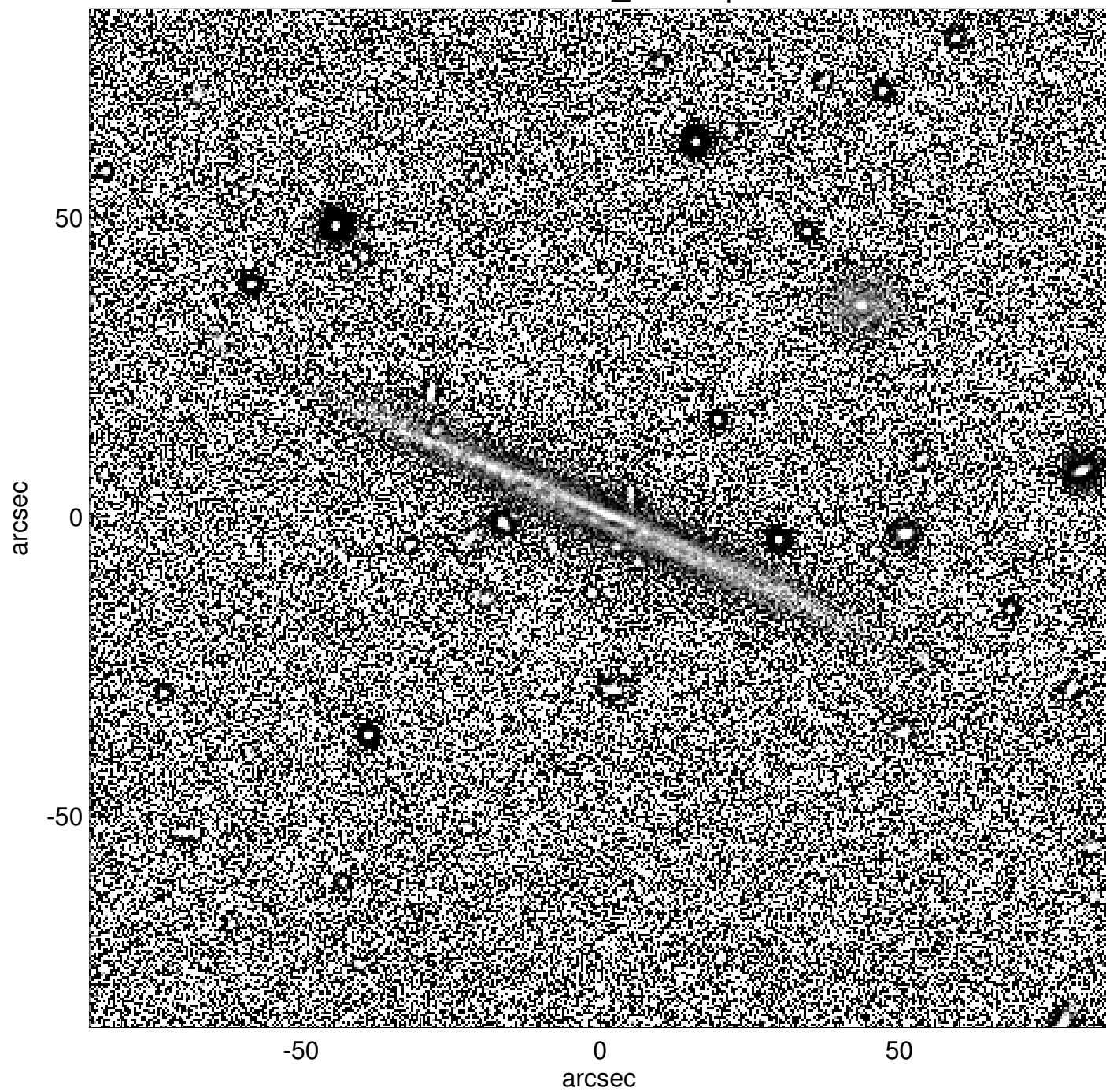
UGC00847_unsharp
