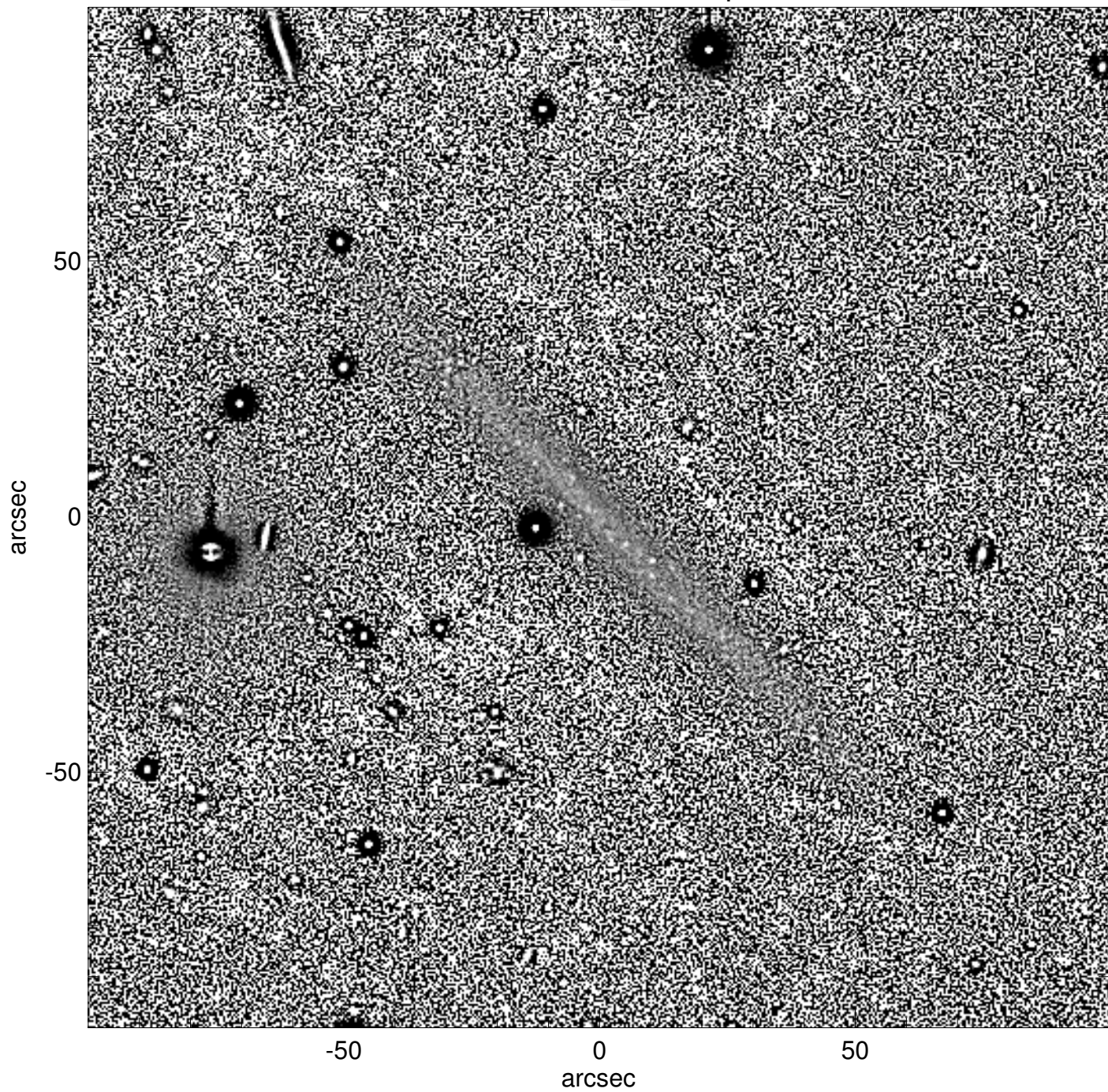
UGC01839_unsharp
