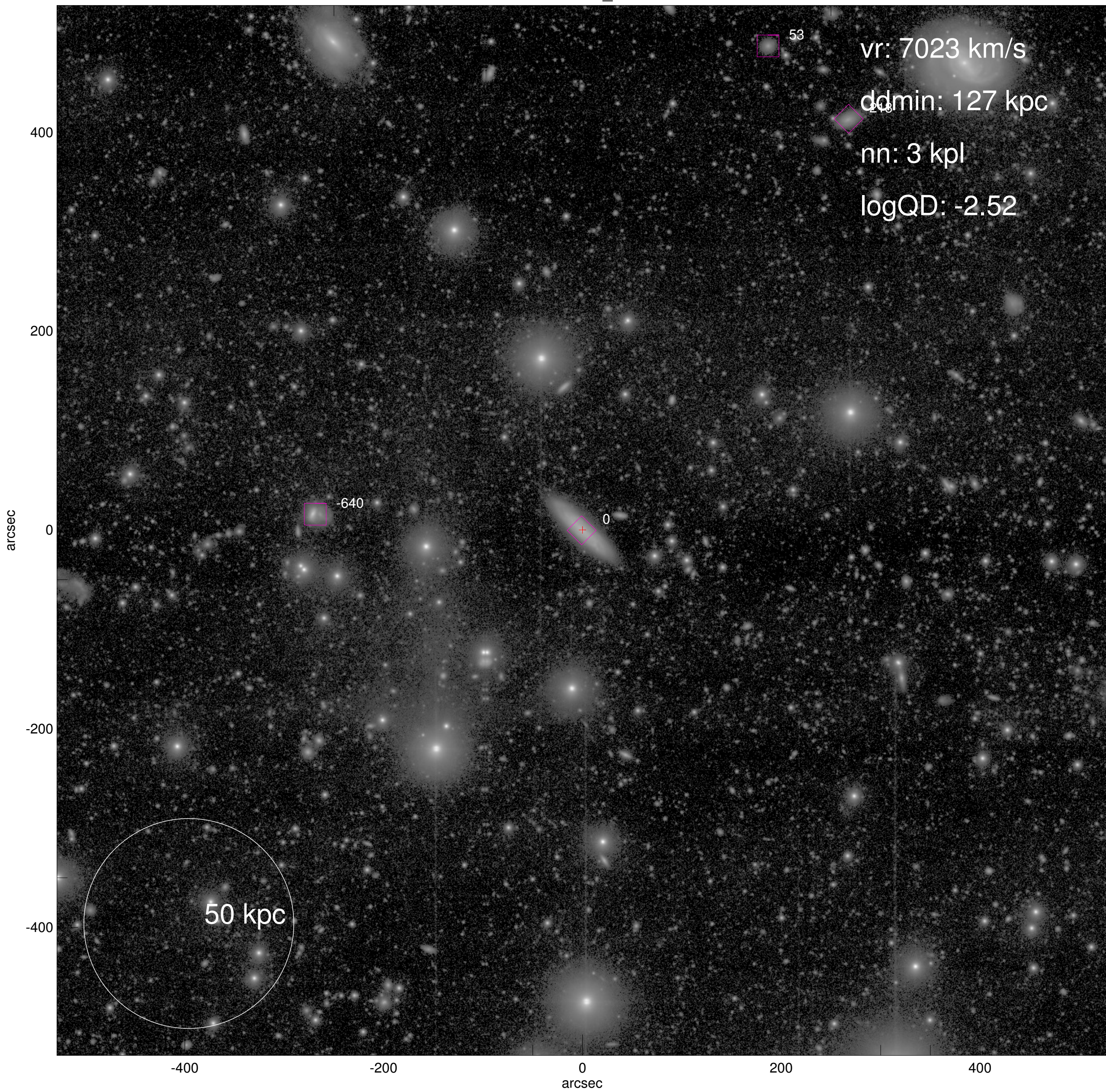
UGC02319_wide
