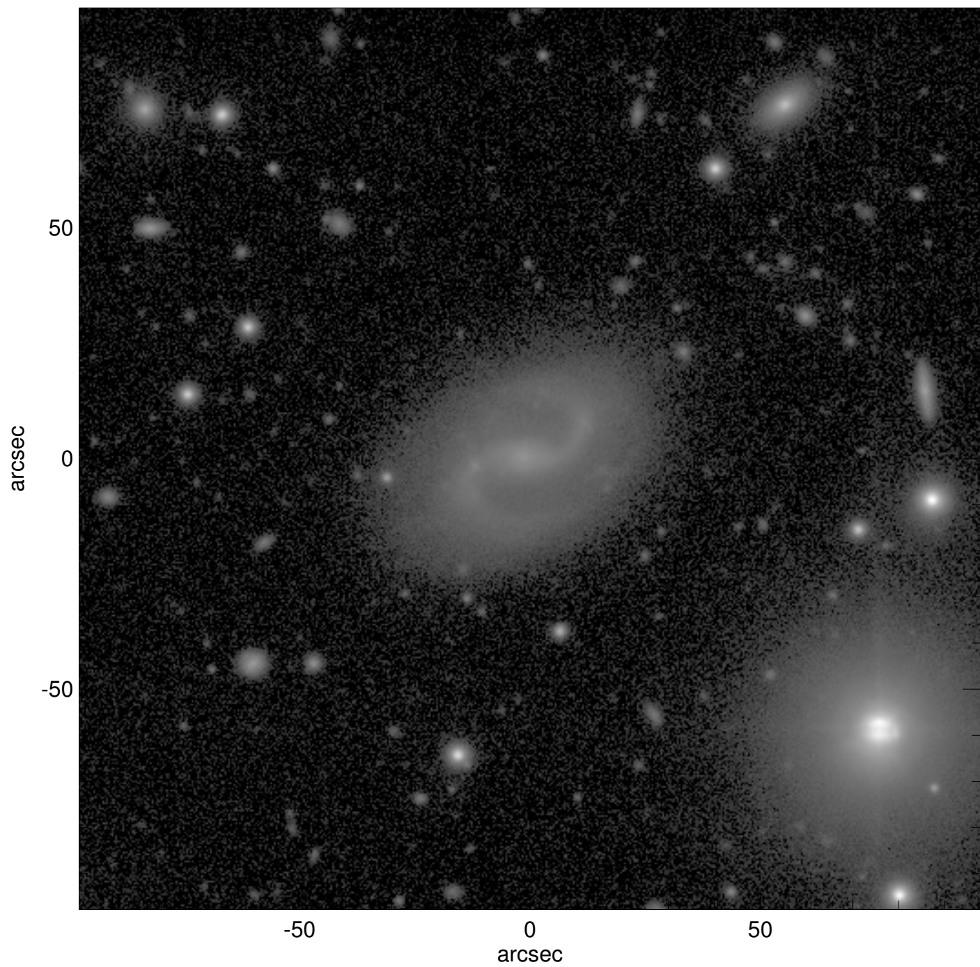
UGC02505
