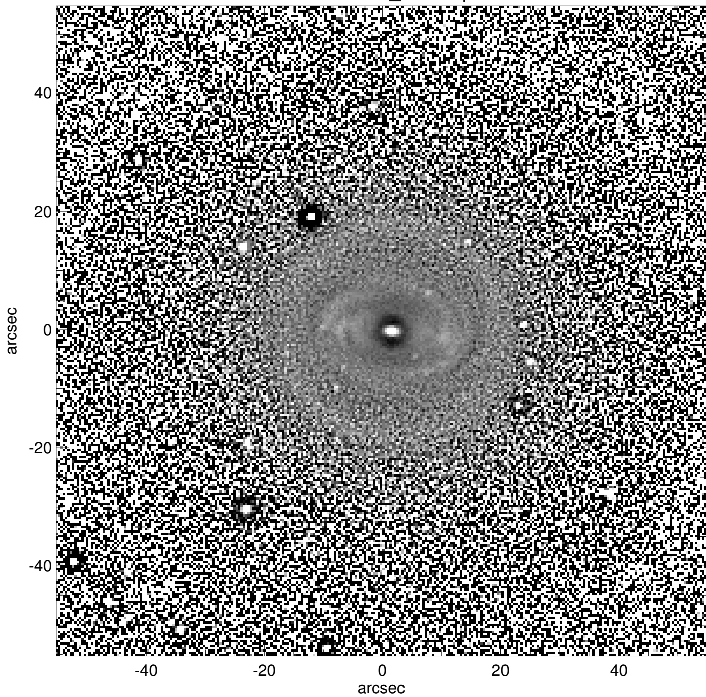
UGC02594_unsharp
