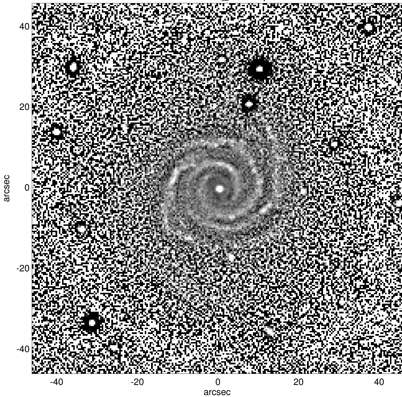
UGC02842_unsharp
