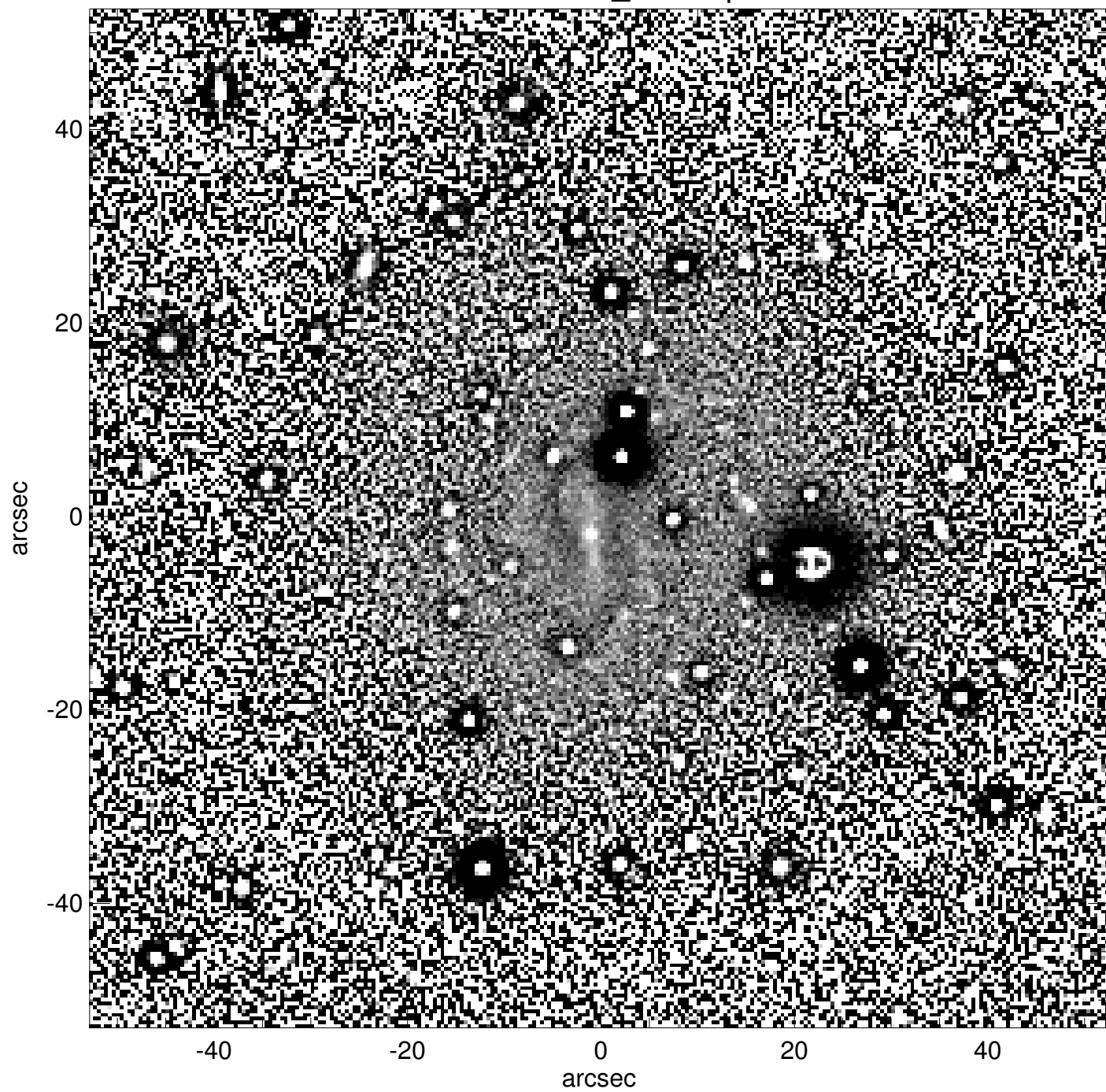
UGC11626_unsharp
