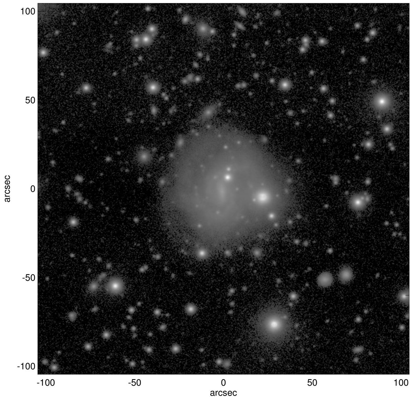
UGC11626
