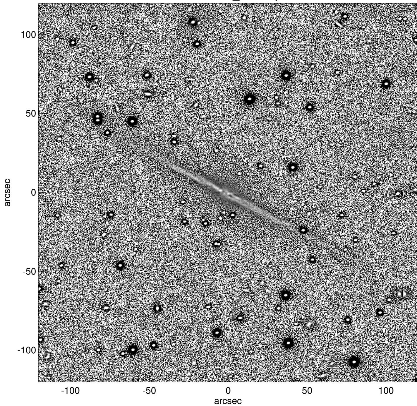
UGC11859_unsharp
