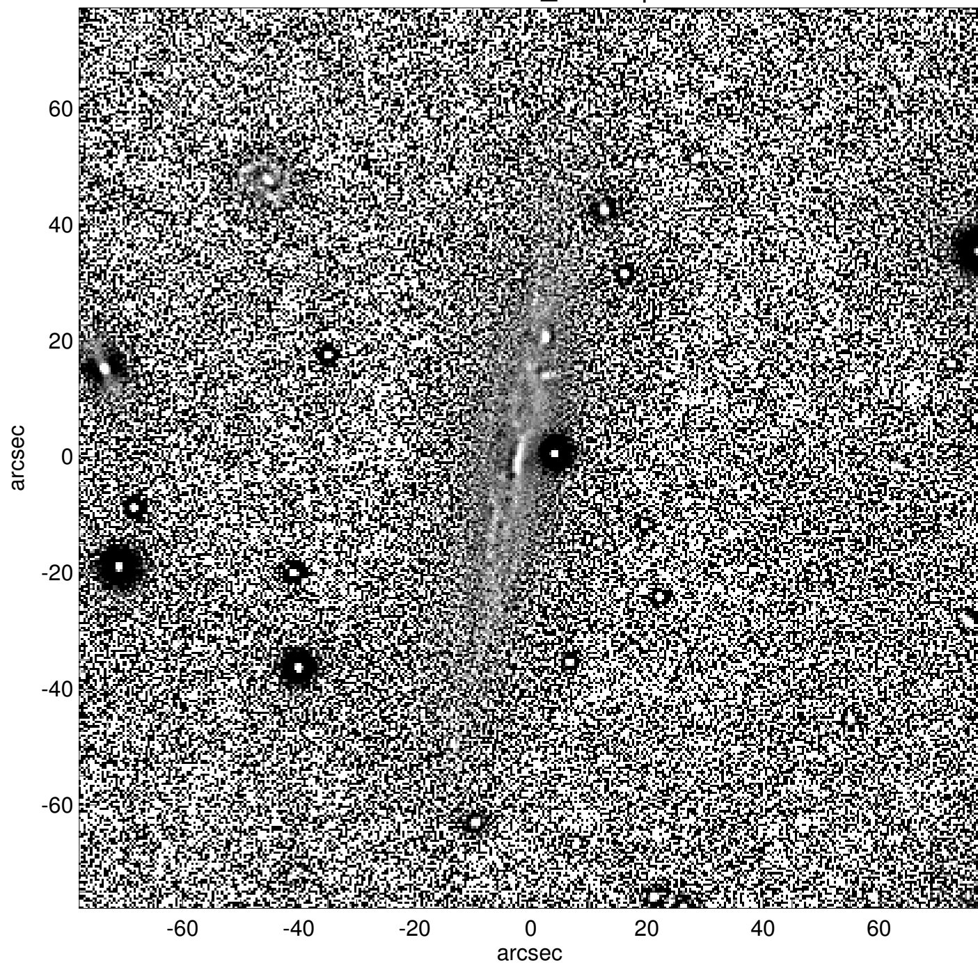
UGC11982_unsharp
