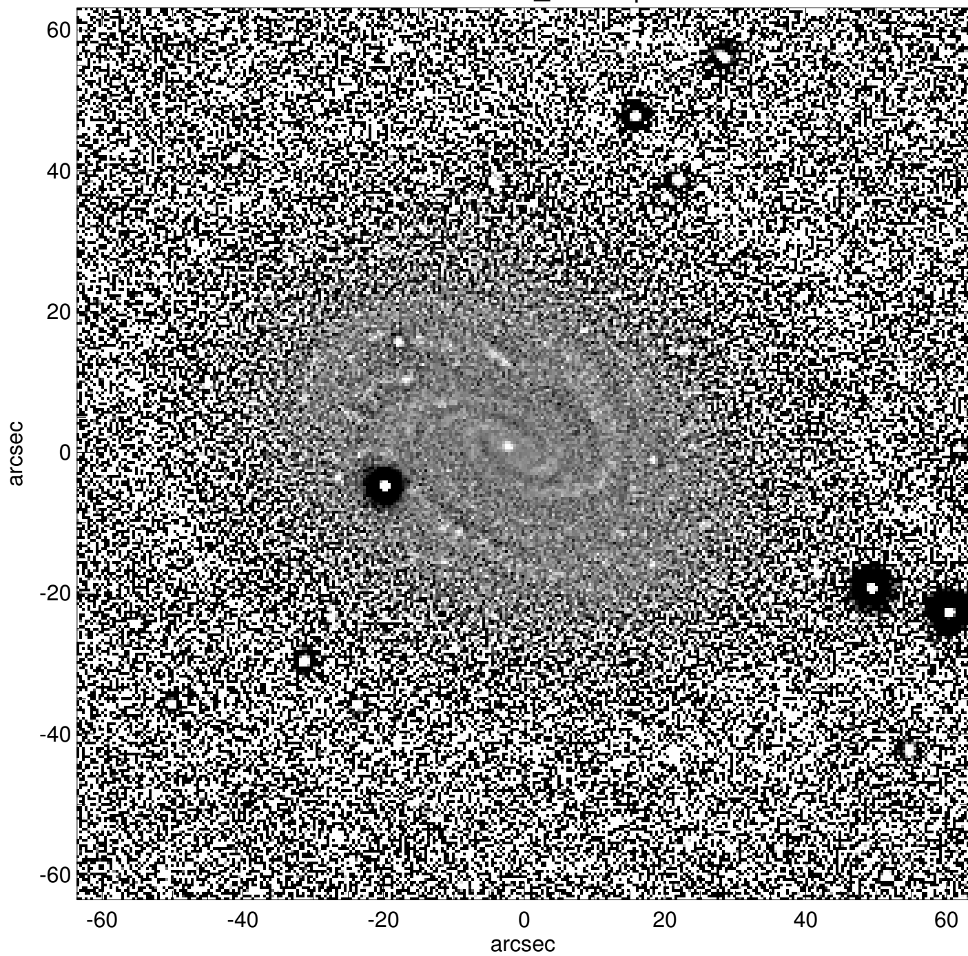
UGC12208_unsharp
