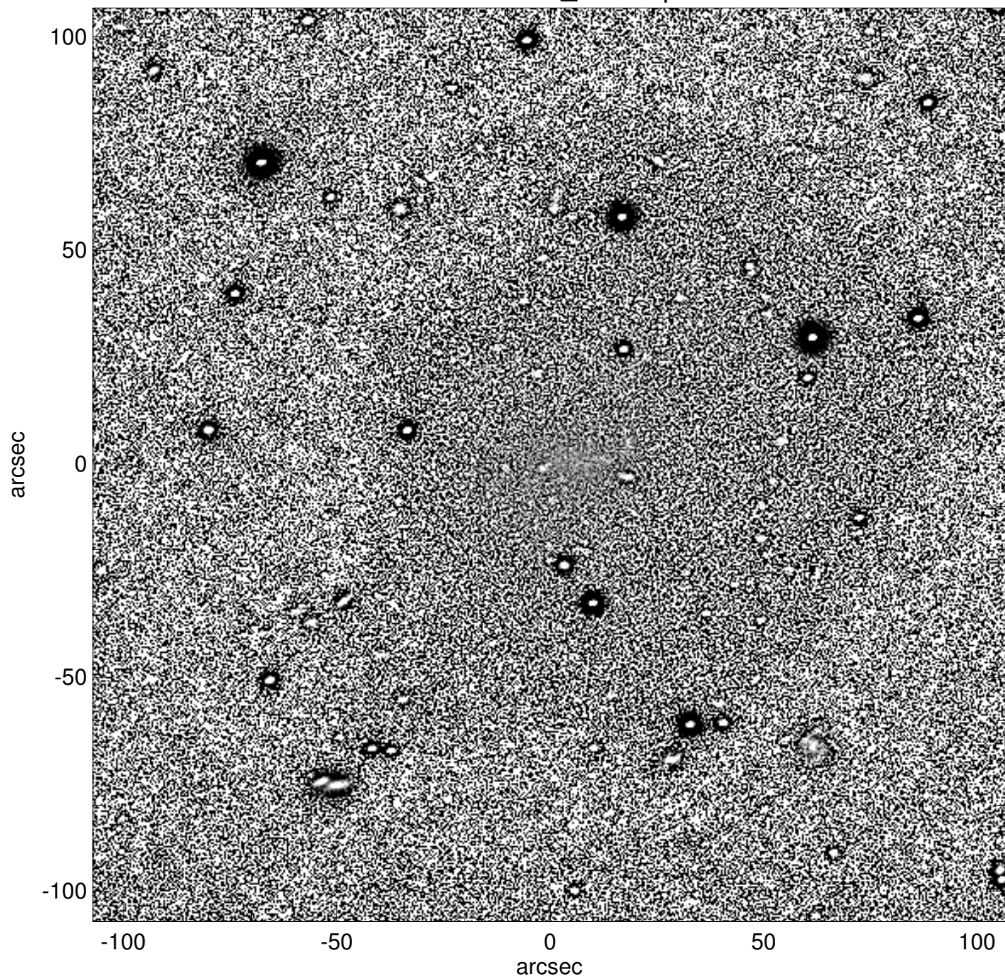
UGC12690_unsharp
