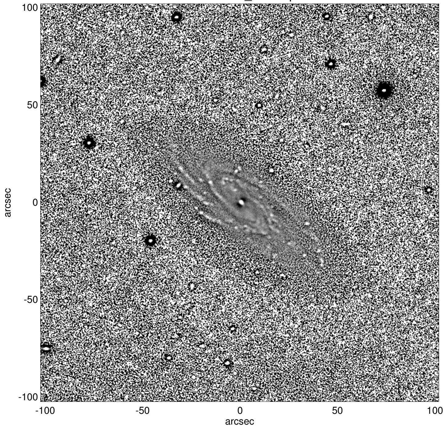
UGC12810_unsharp
