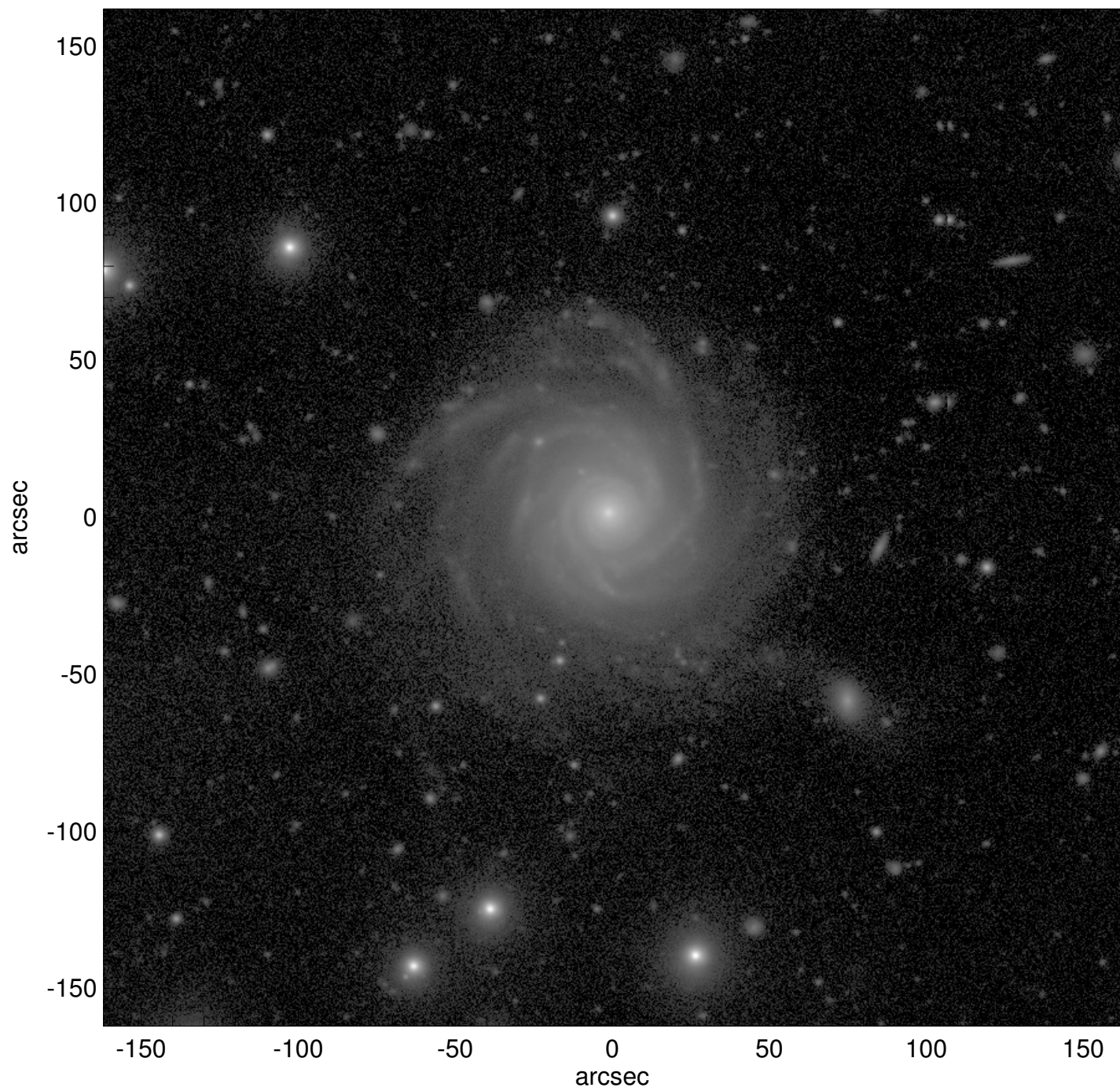
UGC12852
