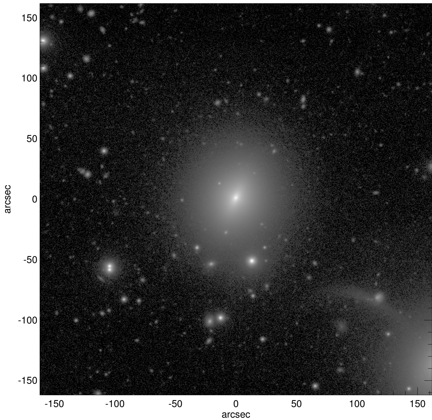
NGC0430
