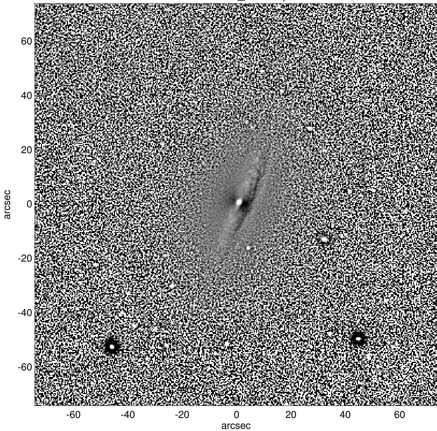
NGC0442_unsharp
