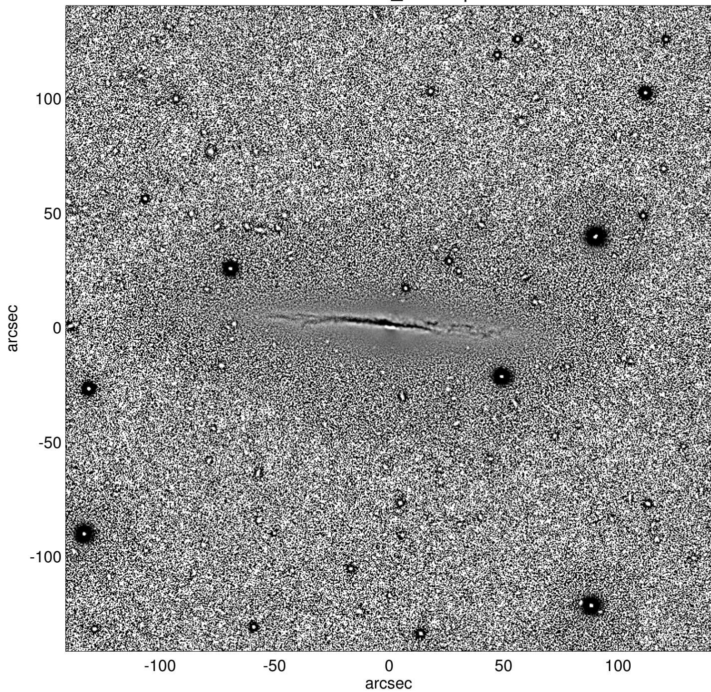
NGC0585_unsharp
